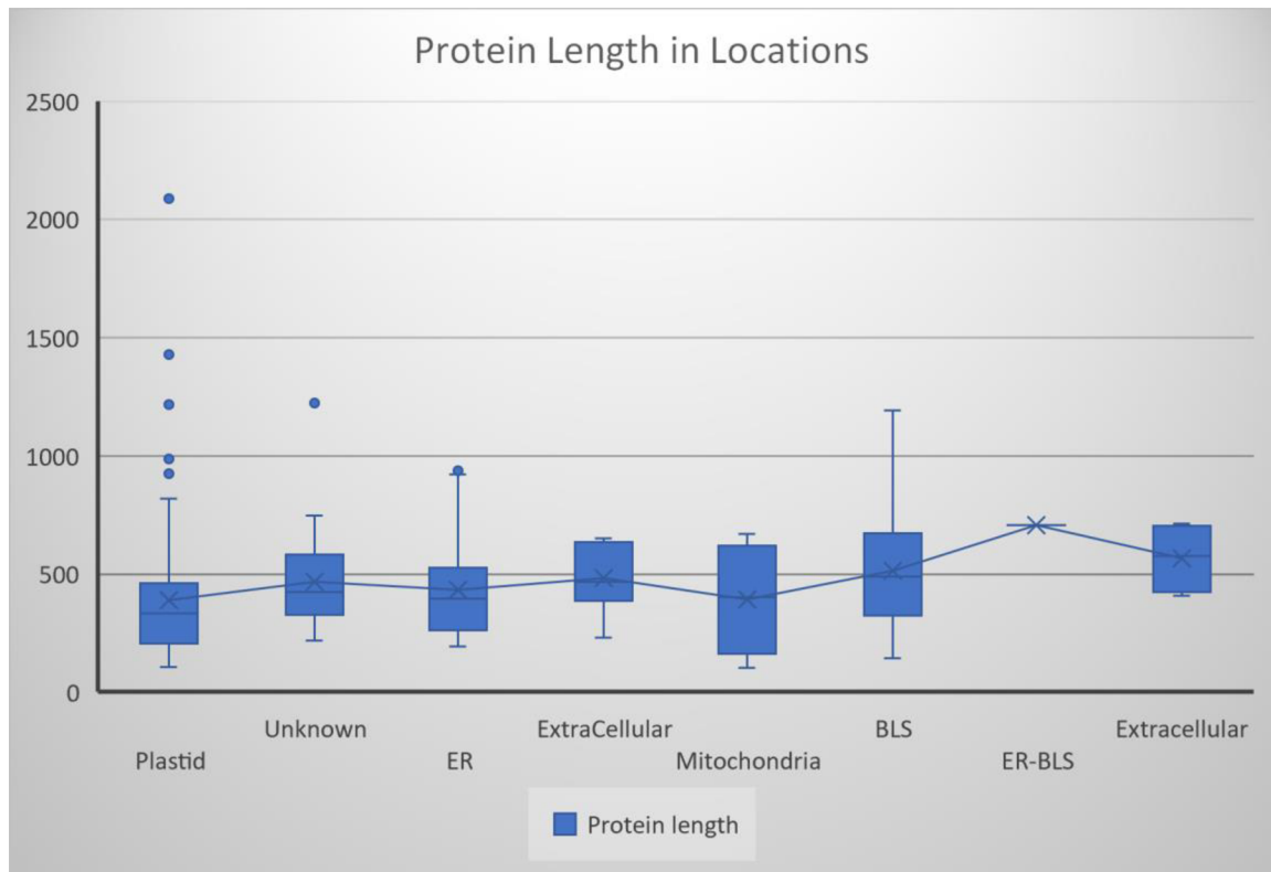
Figure 5: X axis represents the different compartment of the proteins and Y axis represents length of amino acid sequences. Plastid targeted sequences are usually 400 amino acids long, however there, are not much observable differences into other compartments except the ER-BLS. In the dataset has only 1 sequence of ER-BLS sequence, therefore in the graph it just a line and does not have any mean value.
