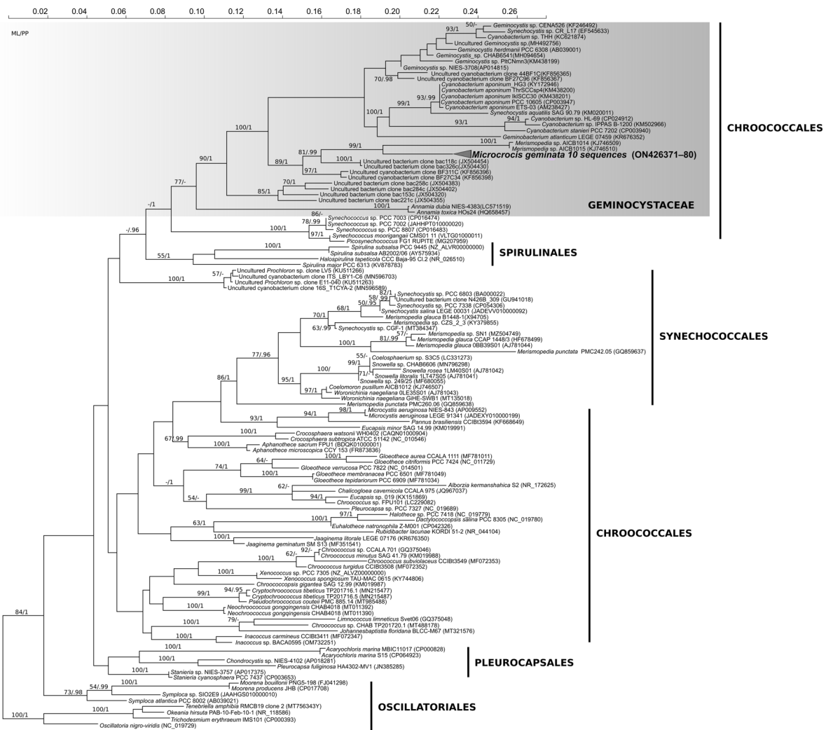
Fig. 3 The phylogenetic tree constructed from the 16S rRNA gene sequences of Chroococcales with a part of Oscillatoriales applied as an outgroup. With the paraphyletic Chroococcales partly interfere the orders Pleurocapsales, Spirulinales and part of Synechococcales, also included in the analyses. Topology represents the best ML tree. Support of bootstrap of Maximum Likelihood analysis above 50 (ML) and posterior probabilities of Bayesian Inference analysis above 0.95 (PP) are recorded. Our 10 sequences of M. geminata are highlighted in bold font.
