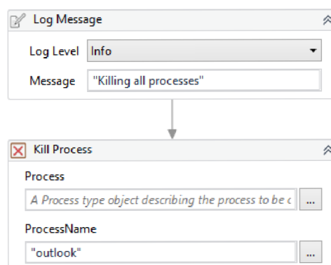
Obr. 5.8: Workflow – KillAllProcesses
