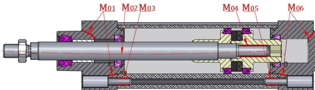
Figure 5.10 Mechanical defects [54].
