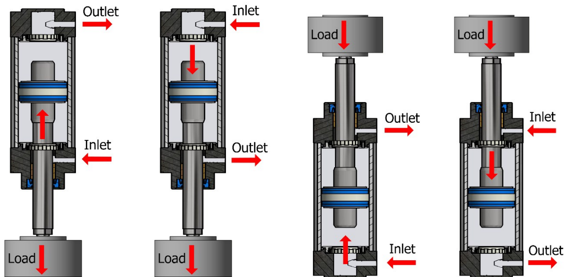
a) Retreat stroke b) Progress stroke c) Progress stroke d) Retreat stroke Load is below piston Load is above piston
