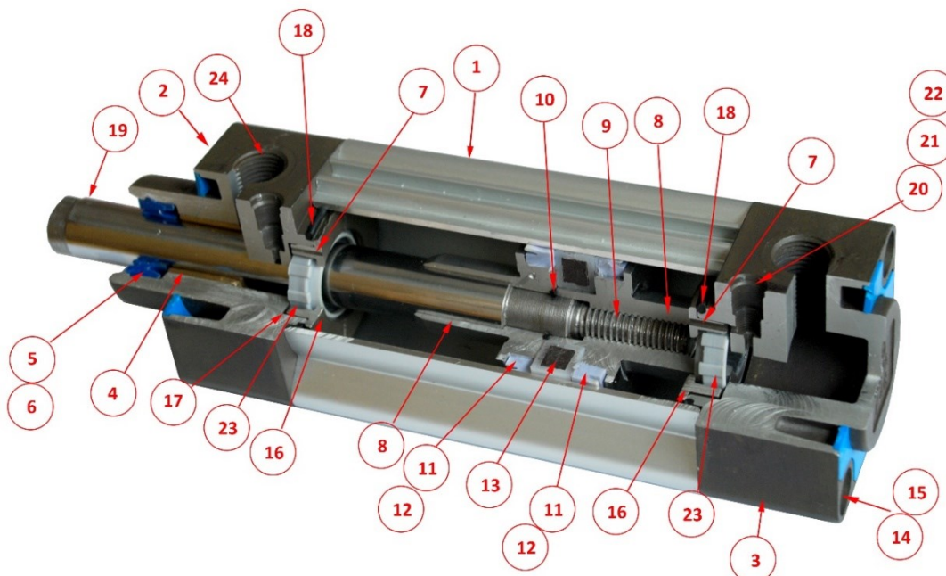
Figure 5.2 Parts of pneumatic cylinder PS.
