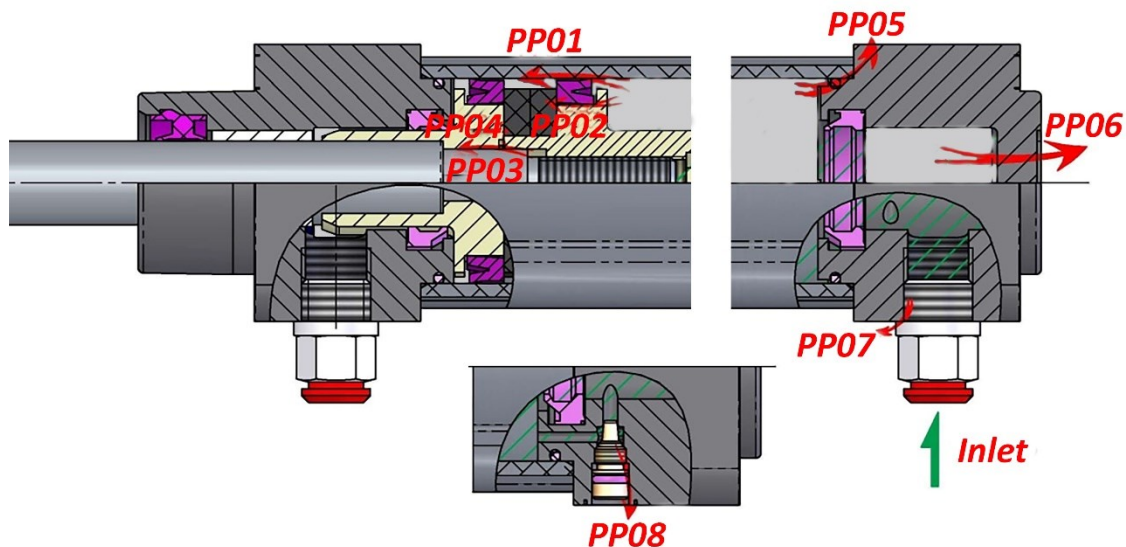
Figure 5.6 Leaks below the piston in the progress stroke [54].
