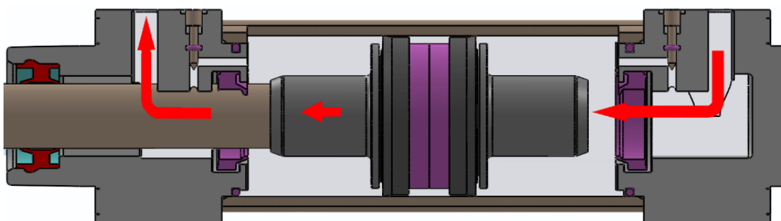
Figure 5.3 Progress stroke steps and position of piston.
