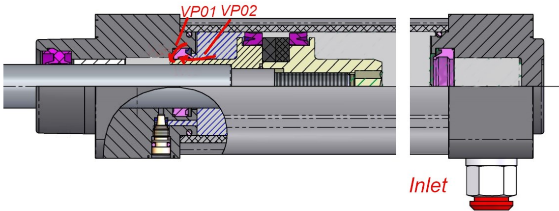
Figure 5.7 Leaks during damping in progress stroke [54].
