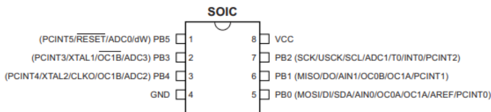
Obr. 3.1: Pinout ATtiny85 [20].
