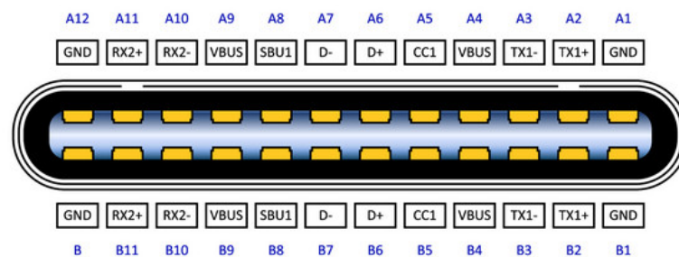
Obr. 1.3: USB-C [5].
