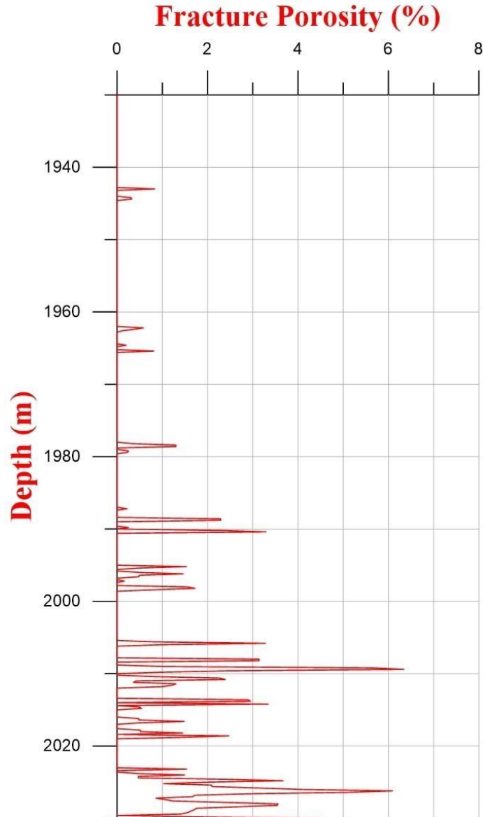
Figure 3.3: Fracture Porosity on Shiranish Formation in the Oil Field
