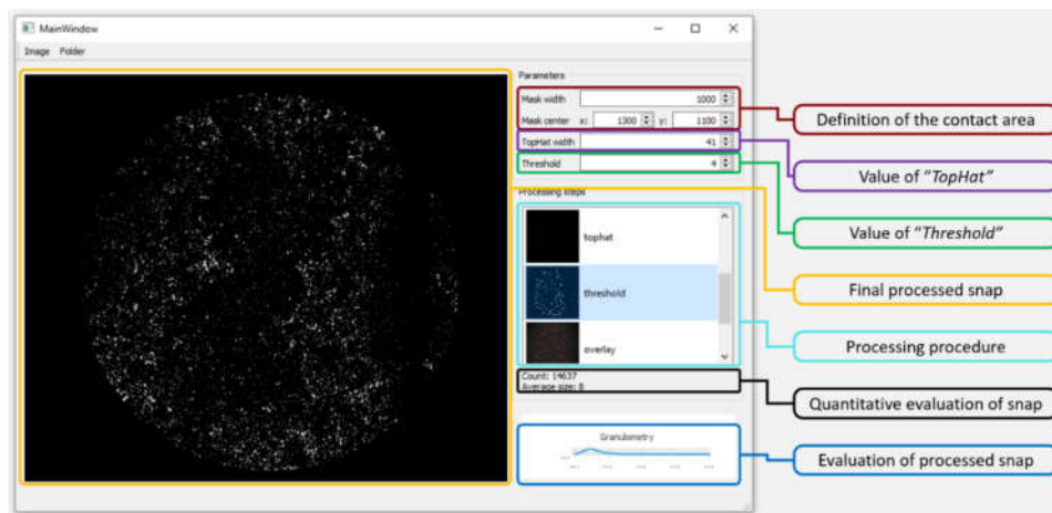
Figure 8. Evaluation software.
