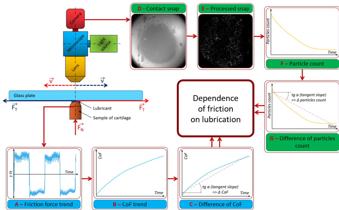
Fig. 5.9 - Evaluation scheme. A - Friction force trend; B - CoF trend; C - Difference of CoF; D - Contact snap; E - Processed snap; F - Particle count; G - Difference of particle count
