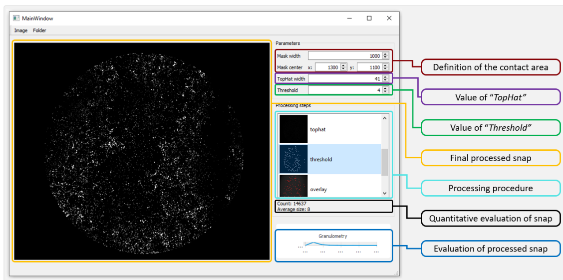
Fig. 5.11 – Evaluation software
