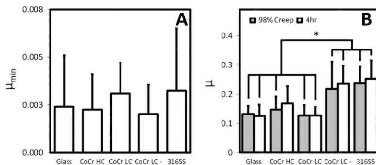
Fig. 2.9 – A – minimal CoF depending on the material; B – CoF in the 98% state of creep and after 4 hour of testing [35]
