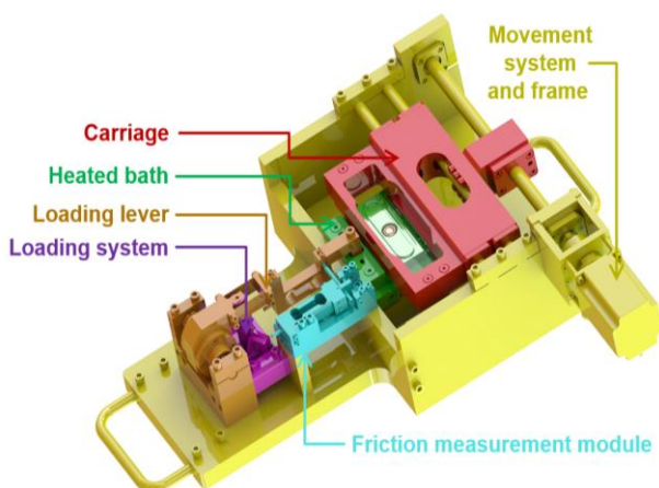
Fig. 2. Real arrangement of apparatus.
