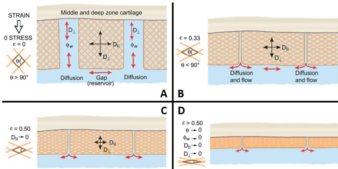
Fig. 2.14 - Compression process [22]
