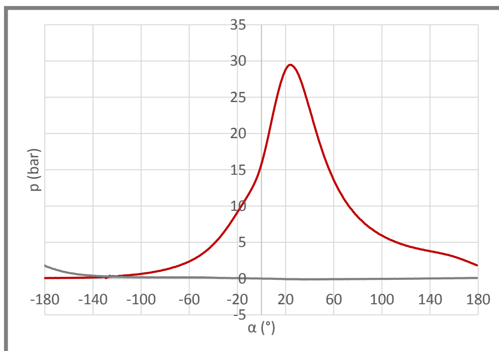
Graf 9 p - \alpha diagram pro n = 2013 \text{ min}^{-1} a 22^{\circ} BTDC
