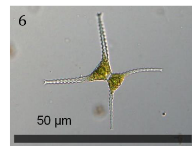
1 – Rhizoclonium sp.; 2 – Closterium moniliferum ; 3 – nahoře Zygnema sp., dole Spirogyra sp.; 4 – Pediastrum duplex ; 5 – Oedogonium sp.; 6 – Staurastrum chaetoceras
