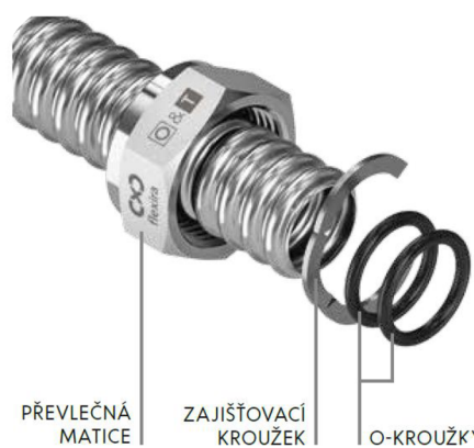
Obr. 1.6: Flexira xConnect System O [8]
