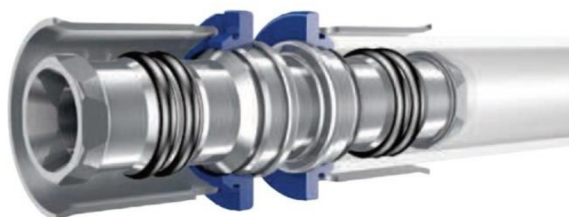
Obr. 1.14: Tvarovka M-press [11]
