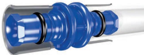
Obr. 1.13: Tvarovka K-press [11]
