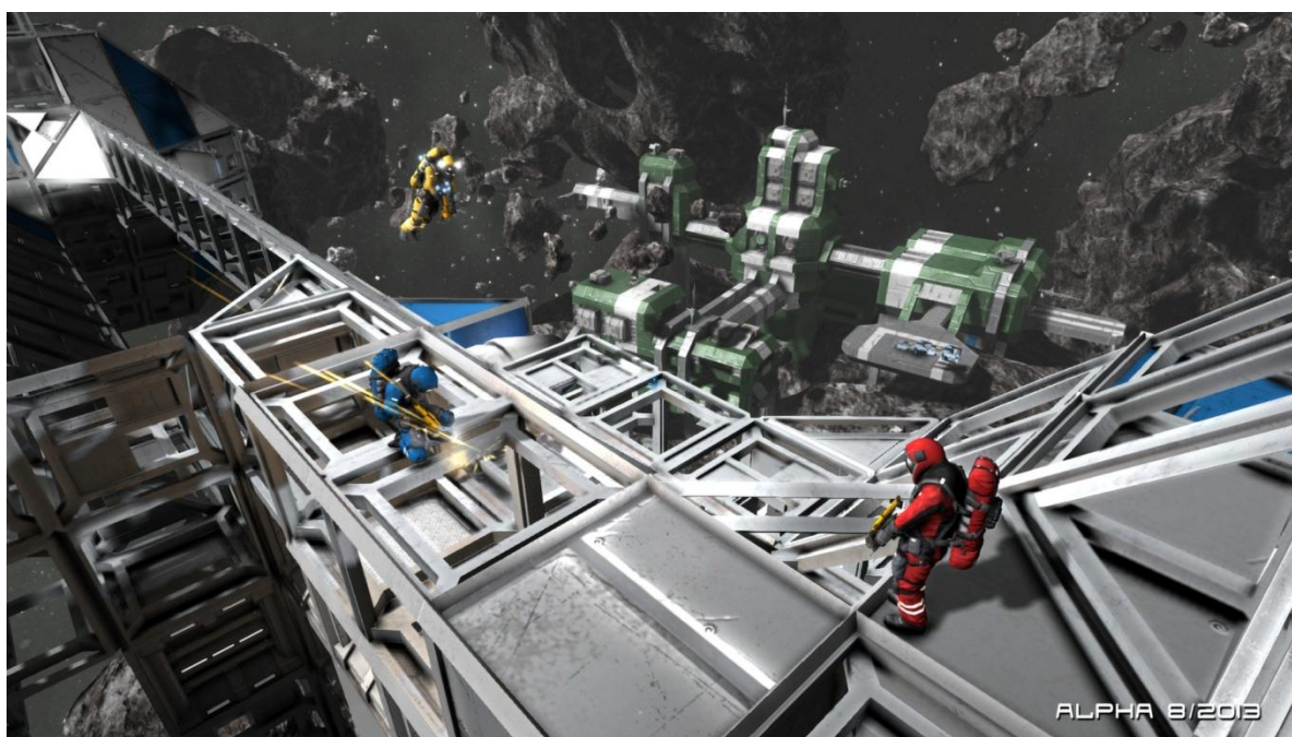
Obr. 5 Space engineers
