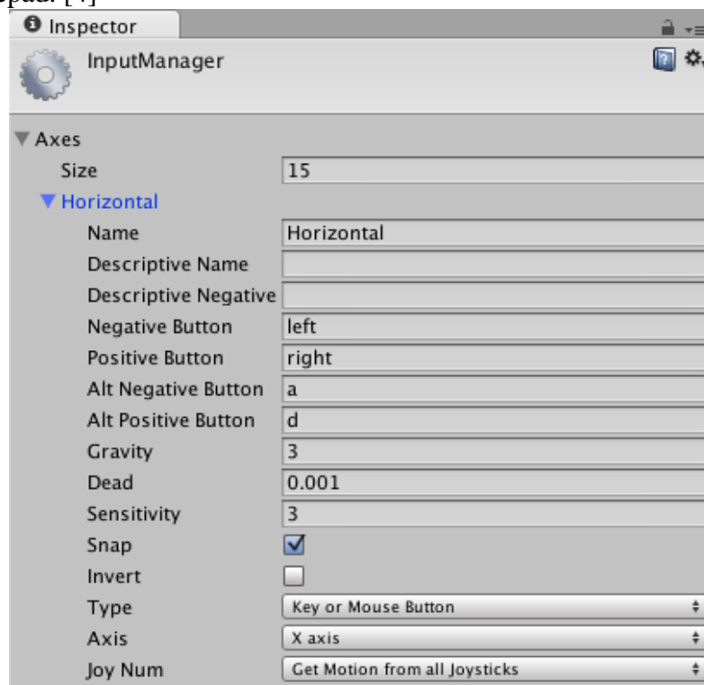
Obr. 11 Input manager
