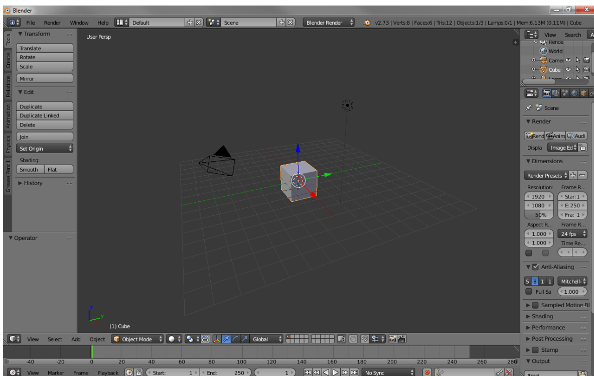
Obr. 16 Blender Editor
