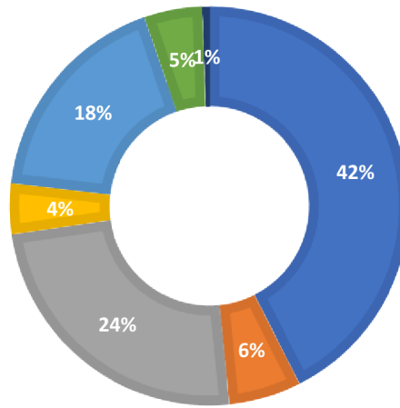
Figure 14. Farmland bird indicator with percentages of abundance for each species in 2023.
