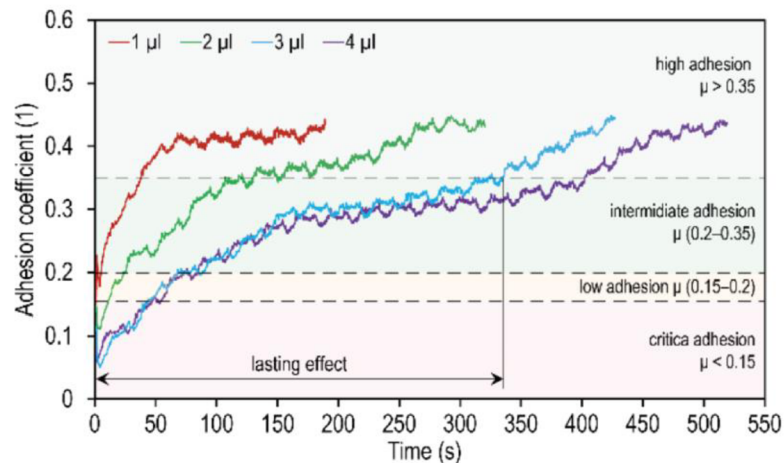
Fig. 2.14 Twin-disc testing of commercial TOR lubricant under different applied amounts [12].
