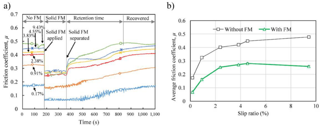
Fig. 2.19 Coefficient of friction for solid FM as a function of: time (a) and slip (b) [37].
