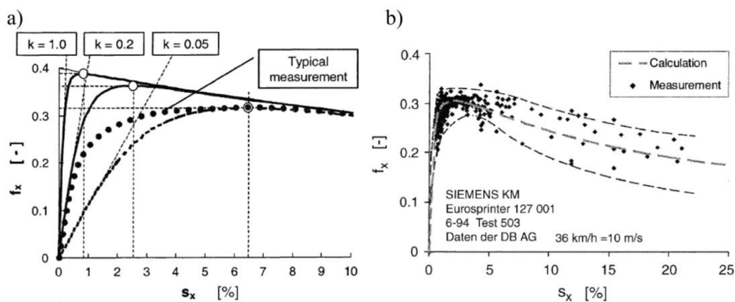
Fig. 2.26 Comparison of single reduction factor for Kalker's coefficients (a), model of traction curve for locomotive Siemens Europrinter 127001 (b) [58]
