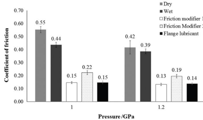
Fig. 2.9 Influence of pressure on tested substances (a), measurement of friction modifier (b) [25].
