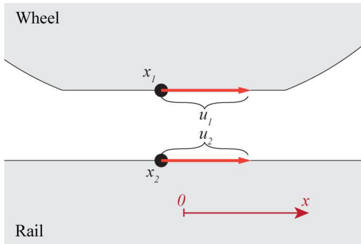
Fig. 5.6 An illustration of contact surface kinematics.
