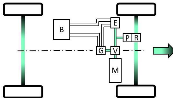
Obr. 1.6 Full hybrid [11]
