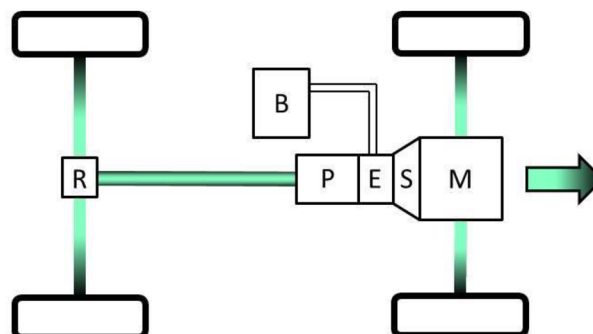
Obr. 1.5 Mild hybrid [5]
