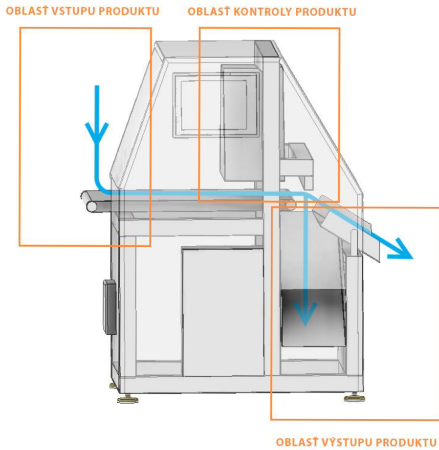
Obr. 2-15 Smer procesu triedenia a oblasti stroja Walso HSI, Krapco
