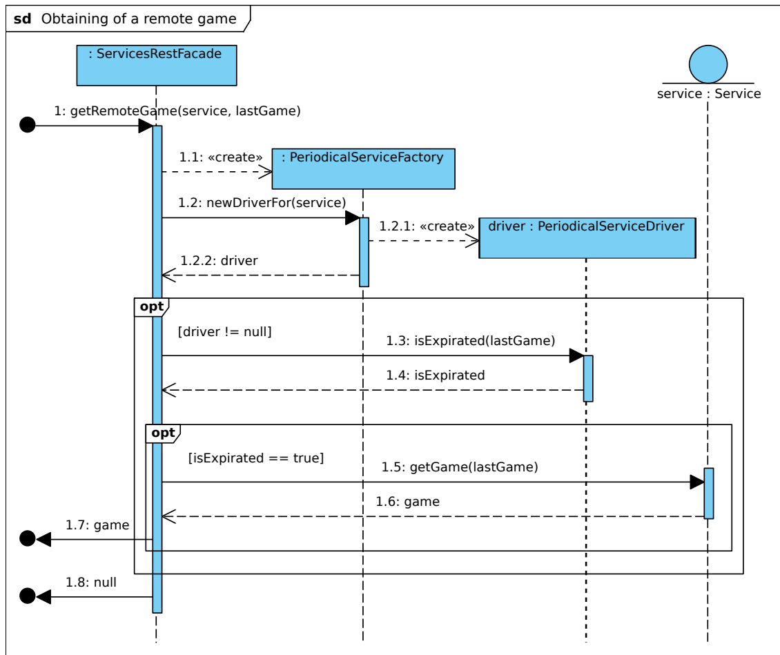
Figure 4.4: The sequence diagram of the getRemoteGame procedure for obtaining of remote published games
