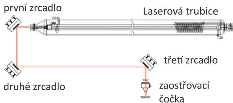
Obr. 10 - Trubice \text{CO}_2 laseru [11]
