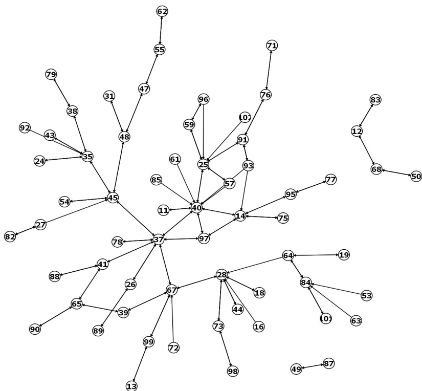
Figure 17: Similarity graph with stretching equal to 1 (economic and financial variables included) (Source: Own work)
