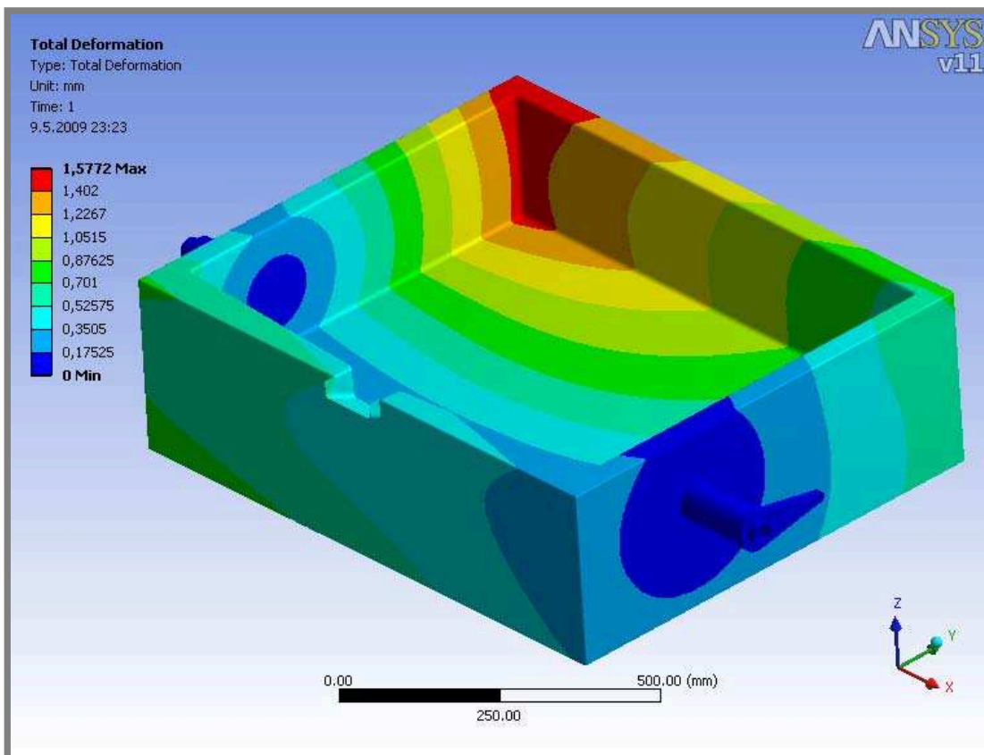
Obr. 6-19 Vana – deformace
