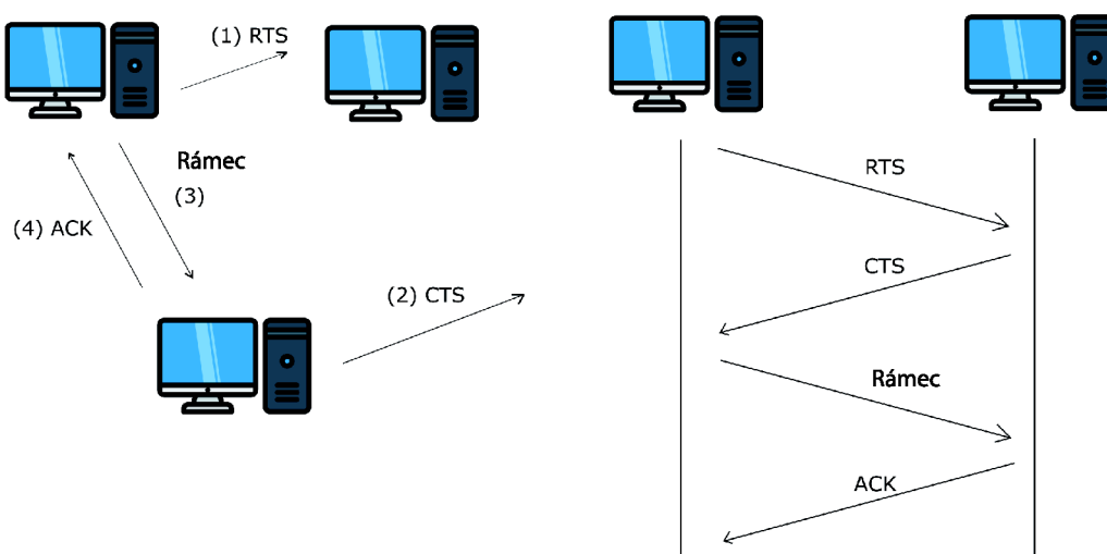
Obr. 1.3: Mechanismus RTS/CTS
