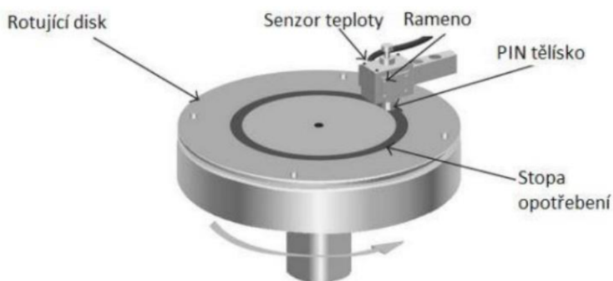
Obr. 2.21 Metoda Ball-on-Disc [49]
