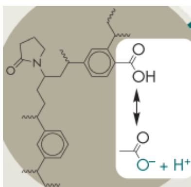
Obr. 40: WCX [131]
