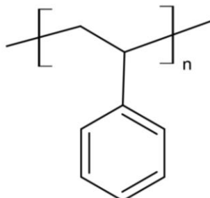
Obr. 36: Sorbent SDB [125]
