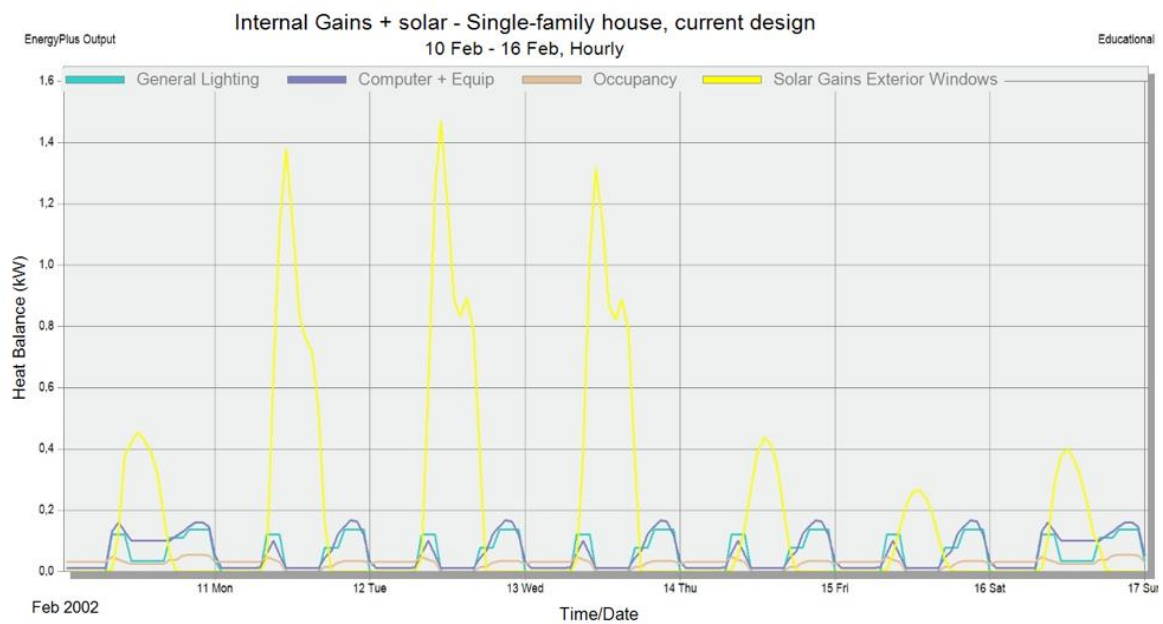
Fig. 11 Internal and solar heat gains for winter design week
