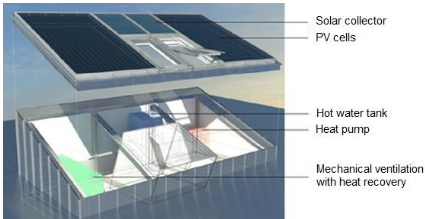
Fig. 5 Detail of the unique prefabricated element [30]
