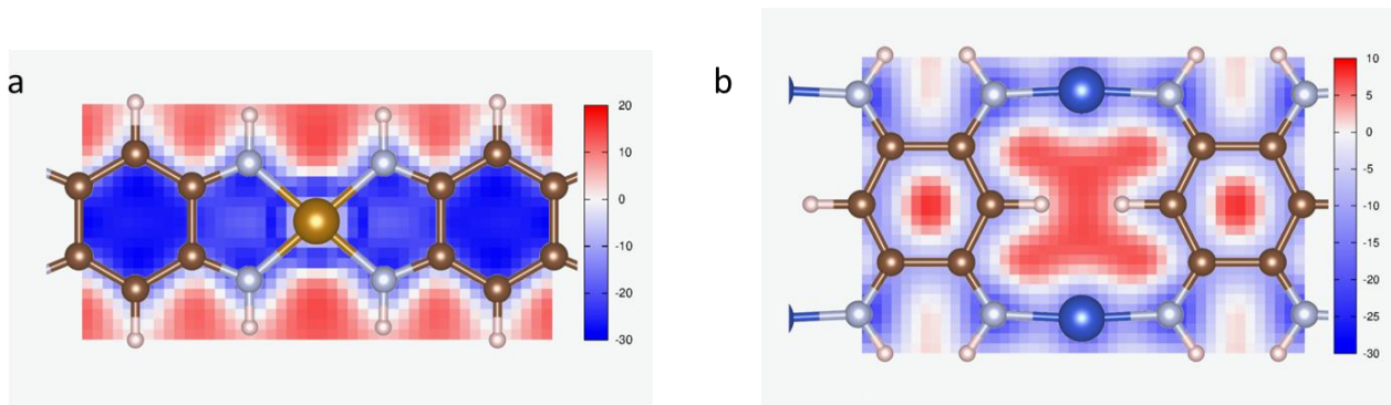
Figure 2.10: (a) NICS grid of FeQDI /Au(111) (b) NICS grid of Cu 2 QDI /Cu(111). Adapted from [71] (Image Courtesy: Adam Matěj)
