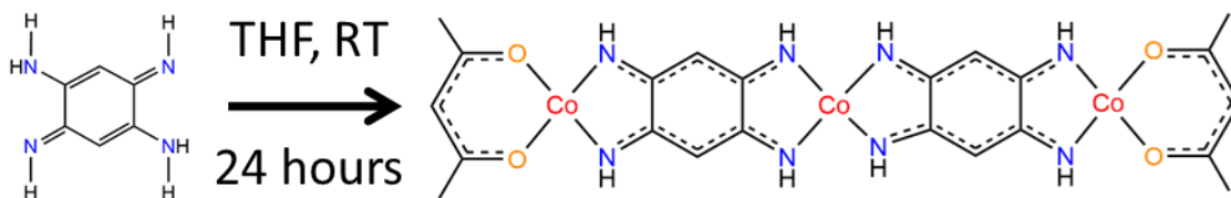
Scheme 5: Synthesis of CoQDI trinuclear complex
