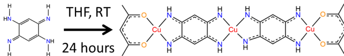
Scheme 6: Synthesis of CuQDI trinuclear complex
