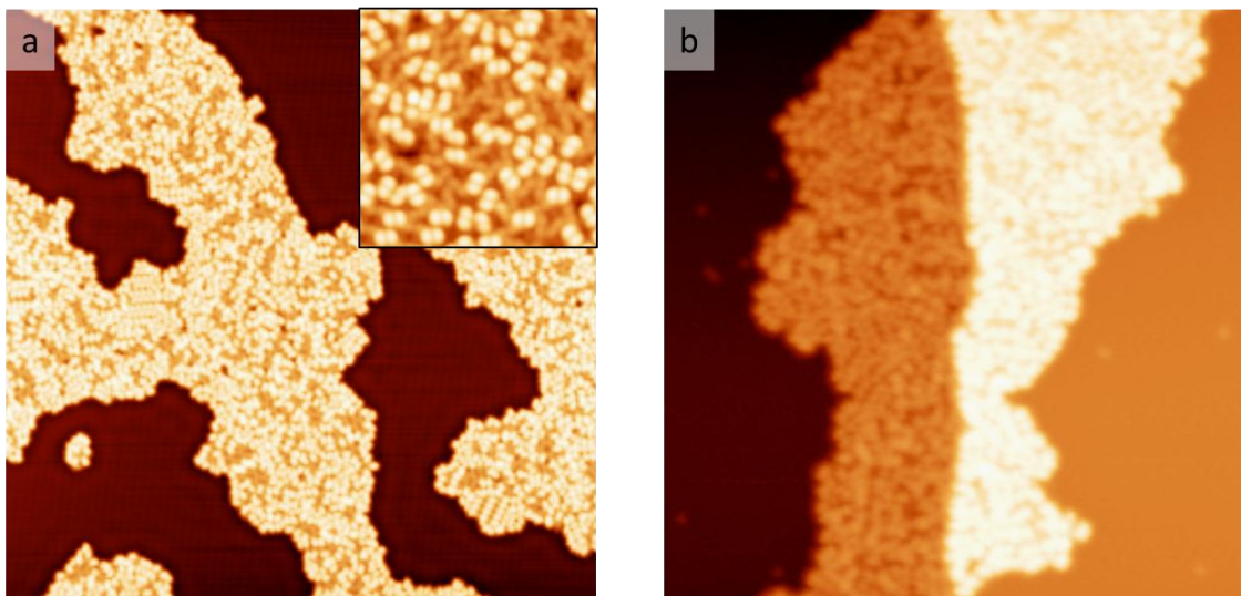
Figure 3.3: Fc 2 -I 2 on Ag(111). (a) STM image of Fc 2 -I 2 islands on surface. (b) STM image of Fc 2 -I 2 islands along the step edges. Scanning Parameters: (a) (500 mV, 10 pA, 100 × 100 nm 2 ); (b) (500 mV, 10 pA, 50 × 50 nm 2 ).
