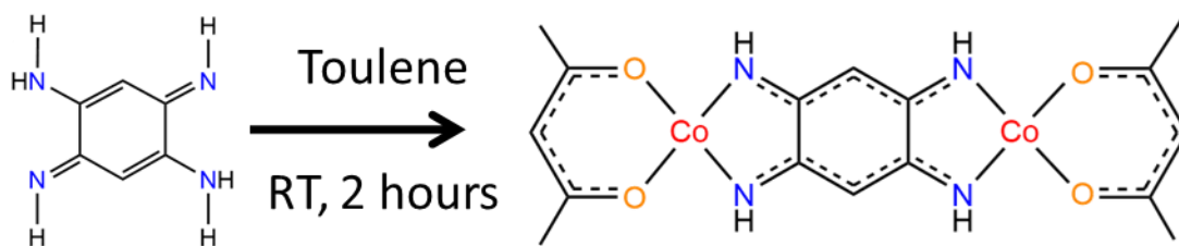
Scheme 2: Synthesis of CoQDI dinuclear complex
