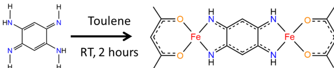
Scheme 1: Synthesis of FeQDI dinuclear complex
