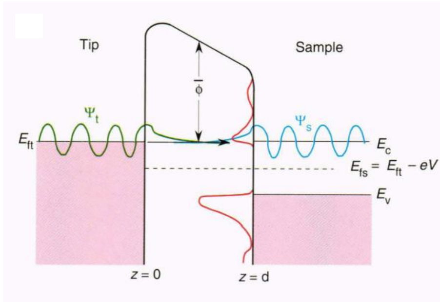
Figure 1.3: Schematic representation of the operational principles that drive a scanning tunneling microscope. Energy E versus distance z of a tunneling junction, where E_f is the Fermi level, E_v is the top of the valence, band E_c is the bottom of the conduction band, \Psi is the electron wave function, and \Phi is the tunneling barrier height. The subscripts t and s refer to tip and sample. The red curves depict the electron density of states of the sample. Adapted from [36]
