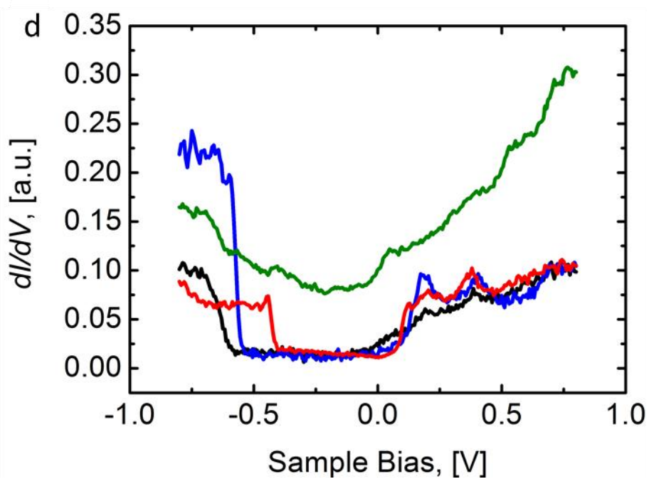
Figure 3.14: dI/dV measured on the two islands (a,b) and the free chain of polyferrocenylene (c). (d) Red, blue, green, and black graphs correspond to measurements on meander island, zig-zag island, inclined configuration and perpendicular configuration of the free chain, respectively. The positions of spectroscopy are marked in (a-c) by crosses of the same color. Scanning Parameters: (a, b) (10 mV, A_{osc} = 50 pm, 2 \times 2 nm 2 ); (c) (10 mV, A_{osc} = 50 pm, 8 \times 4 nm 2 ).
