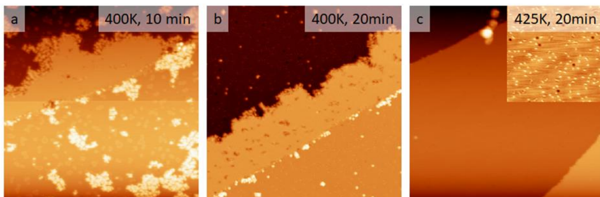
Figure 3.5: STM topographies of polyferrocenylene samples prepared at different annealing temperature/time on Ag(111). (a) Annealing temperature: \sim 400\text{K} , 10min: some polyferrocenylene nanowires, but also high amount of unordered ferrocene clusters on the surface. (b) Annealing temperature: \sim 400\text{K} , 20min: majority of the ferrocene forms ordered polyferrocenylene nanowires. (c) Annealing temperature \sim 425\text{K} , 20 min: ferrocene desorbs from the surface, only Iodine remains. Scanning Parameters: (a) (900 mV, 10 pA, 100 \times 100 \text{ nm}^2 ); (b) (500 mV, 10 pA, 100 \times 100 \text{ nm}^2 ); (c) (500 mV, 10 pA, 100 \times 100 \text{ nm}^2 ), inset: 50 \times 50 \text{ nm}^2 .
