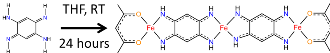
Scheme 4: Synthesis of FeQDI trinuclear complex
