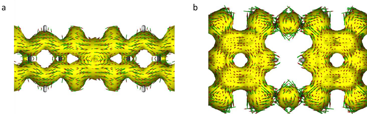
Figure 2.9: (a) ACID plot of FeQDI /Au(111), black arrow indicating the clockwise direction of current density vectors for better clarity. (b) ACID plot of Cu 2 QDI /Cu(111), black arrow indicating the clockwise direction of current density vectors for better clarity. The molecular planes are placed perpendicular to the magnetic field vector. Small green arrows are computed current density vectors. Adapted from [71] (Image Courtesy: Adam Matěj)
