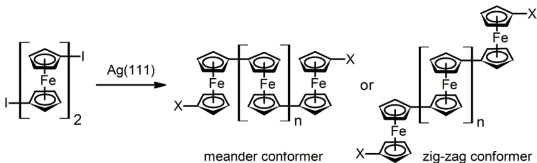
Figure 3.2: Scheme of on surface synthesis of polyferrocenylene on Ag (111) surface. Adapted from [89]
