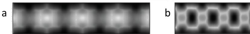
Figure 2.8: Simulated AFM images of (a) FeQDI /Au(111) (b) Cu 2 QDI /Cu(111) coordination polymers. Adapted from [71] (Image Courtesy: Martin Ondraček)
