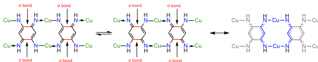
Figure 2.11: Scheme depicting the bonds and resonating structures of the 12 membered macrocycle in Cu 2 QDI wires on Cu(111). Adapted from [71] (Image Courtesy: Olivier Siri)
