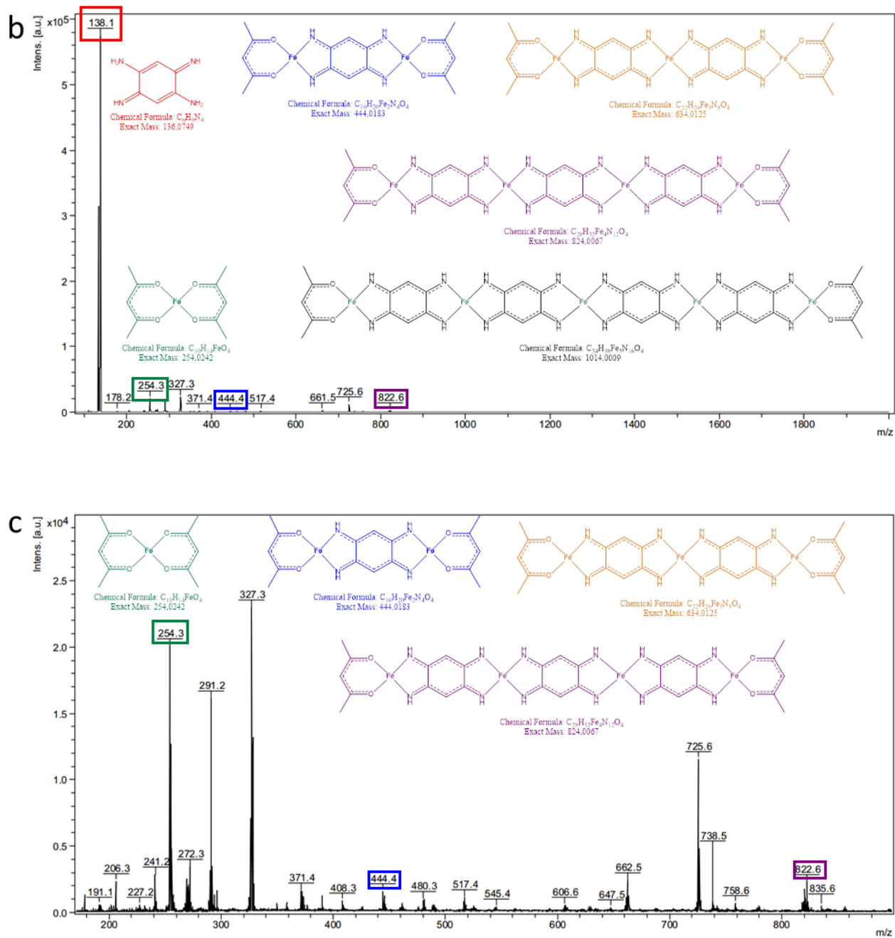
Figure 3: (a) UV-Vis-NIR absorption studies of FeQDI dinuclear complex in DMSO. (b) MALDI Analysis (Positive). (c) Zoom-in MALDI spectra
