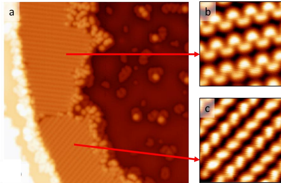
Figure 3.7: (a) STM overview of the two different polyferrocenylene islands. (b, c) Zoom in images of the polyferrocenylene nanowires in the two islands. Scanning Parameters: (a) (-100 mV, 20 pA, 40 \times 40 \text{ nm}^2 ); (b) and (c) constant height current images: 1 mV, 3 \times 3 \text{ nm}^2 . Adapted from [89]
