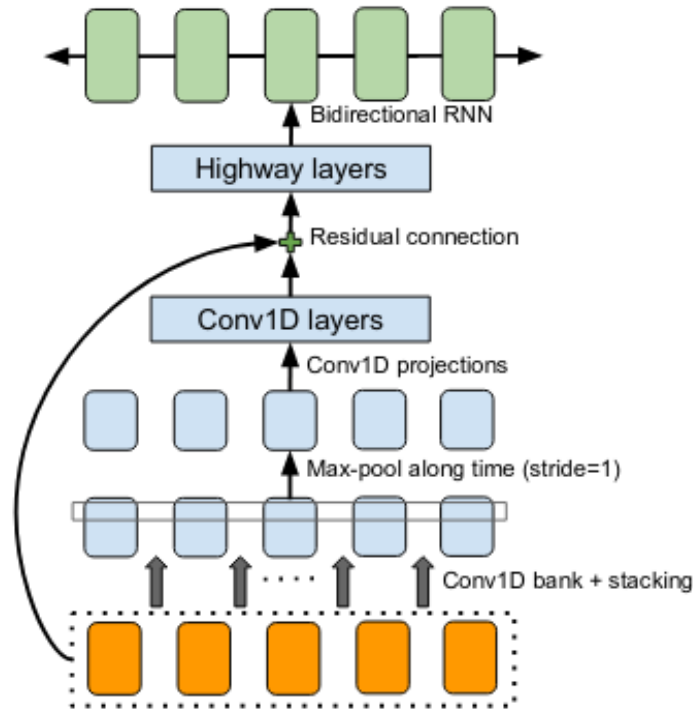
Figure 6.2: The CBHG (1-D convolution bank + highway network + bidirectional GRU) module [19].
