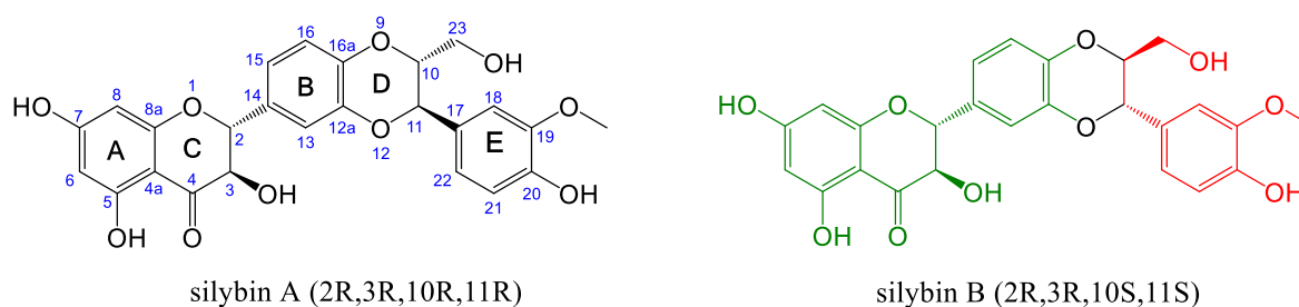
Figure 1. Structure of silybin A and silybin B with the nomenclature. Green and red colors are used to distinguish the flavonoid and the lignan moieties, respectively.
