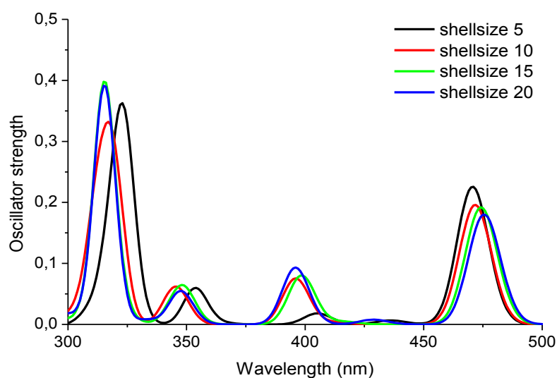
Figure 28. Theoretical absorption spectra of cyanidin-3- O -glucoside···quercetin with four different size of solvation.
