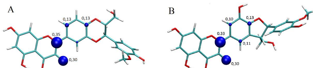
Figure 12. Spin density distribution of the radical formed after hydrogen atom abstraction from the C3-OH group of (A) DHSB and (B) DHSCH.
