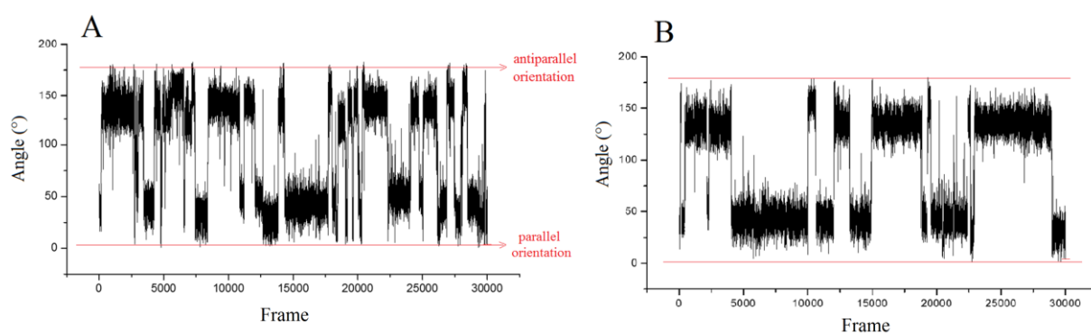
Figure 13. Changes between parallel ( 0^\circ ) and antiparallel ( 180^\circ ) orientations of A) cyanidin-3- O -glucoside: quercetin ( \alpha_2 ) and B) malvidin-3- O -glucoside: quercetin ( \alpha_2 ) within 300 ns MD simulation (1 frame corresponds to 10 ps).
