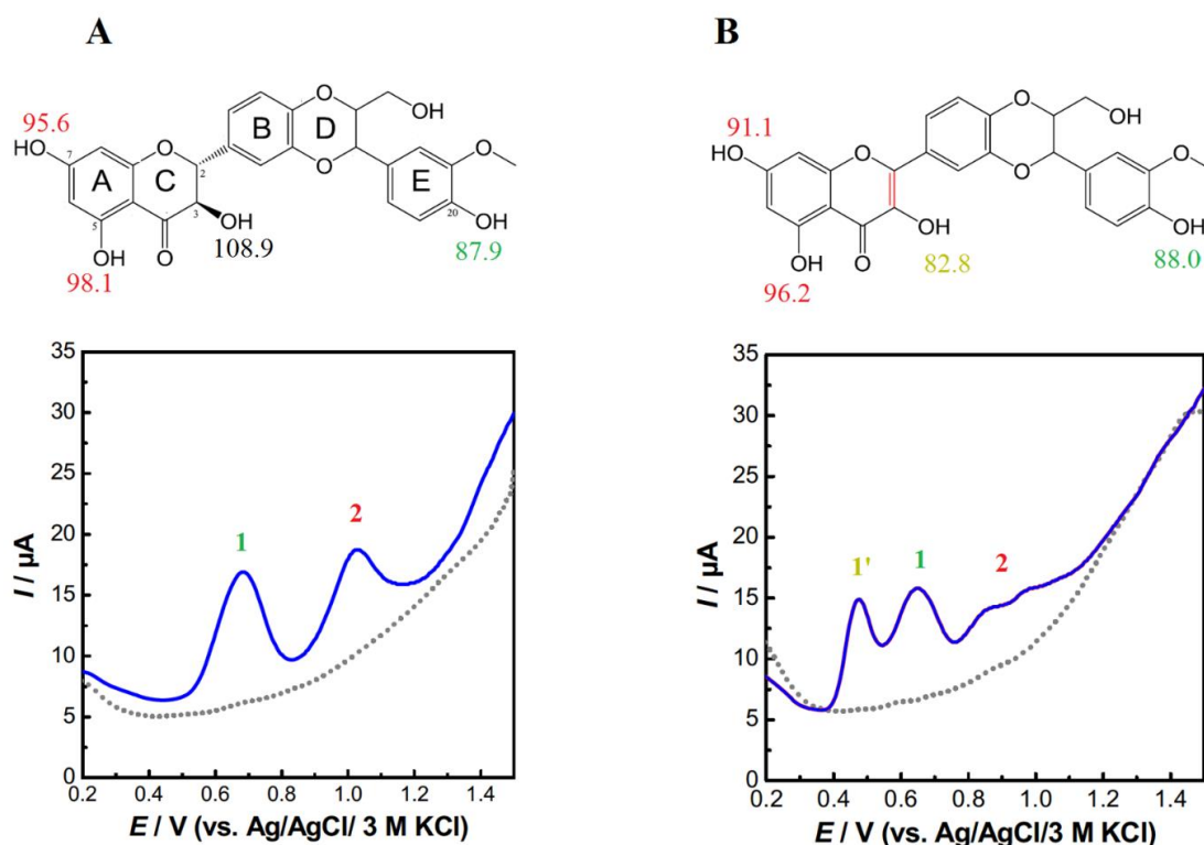
Figure 4. Voltammograms and structures of (A) SB and (B) DHSB. The BDE values of each OH group are expressed in kcal/mol next to the OH groups. The color of the value corresponds to the color of the oxidation peak's number.
