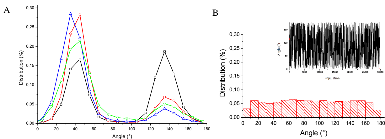
Figure 14. \alpha_2 -distribution of malvidin-3- O -glucoside and quercetin (black), isorhamnetin (red), kaempferol (blue) and galangin (green). Malvidin-3- O -glucoside···caffeine system. B) \alpha_1 angle. Inset: Frequency of the switch between parallel and antiparallel orientations.
