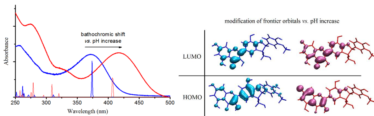
Figure 7. Superimposed theoretical and experimental absorption spectra of DHSCH vs. pH (on the left) and MOs description of the neutral and C7-OH deprotonated form in the first and second column, respectively, on the right. The blue color (spectrum on the left and MOs on the right) corresponds to the neutral form; the red color corresponds to the C7-OH deprotonated form.
