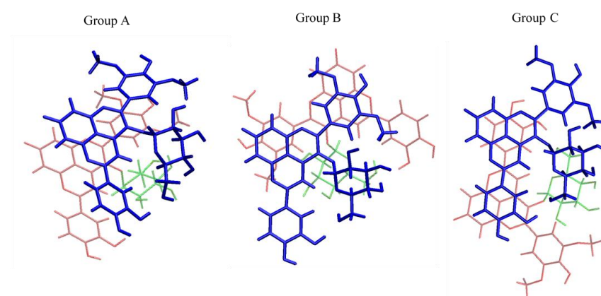
Figure 9. Three representative conformers of PA1 \cdots PA1 dimers. Group A: interactions between A-, C-, D- rings of both PA1 fragments; Group B: interactions between A-, C-, D- rings of one PA1 and the B ring of the other PA1 and Group C: interactions between A-, C-, D- rings of one PA1 with the E ring of the other PA1. For clarity, one PA1 partner is in blue, the other is in red and the sugar moiety is in green.
