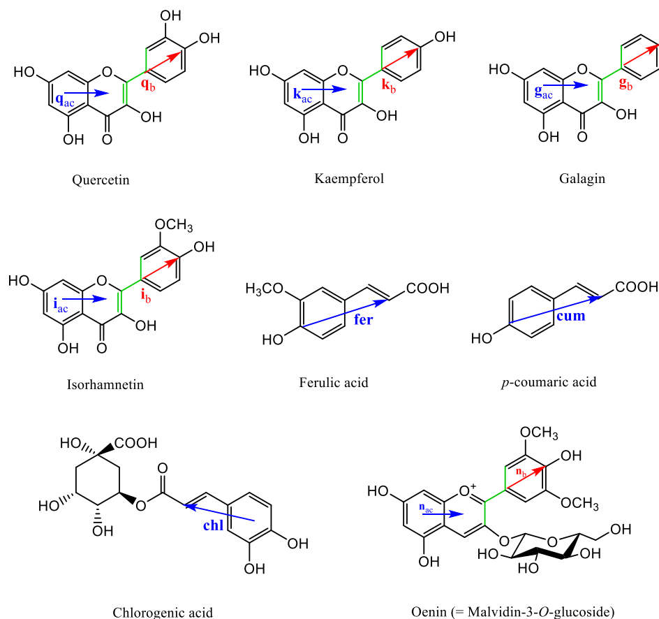
Figure 11. Structures of the pigment and copigments. Vectors within the A-, C-rings and B-ring are in blue and red color, respectively. Dihedral angles are in green.
