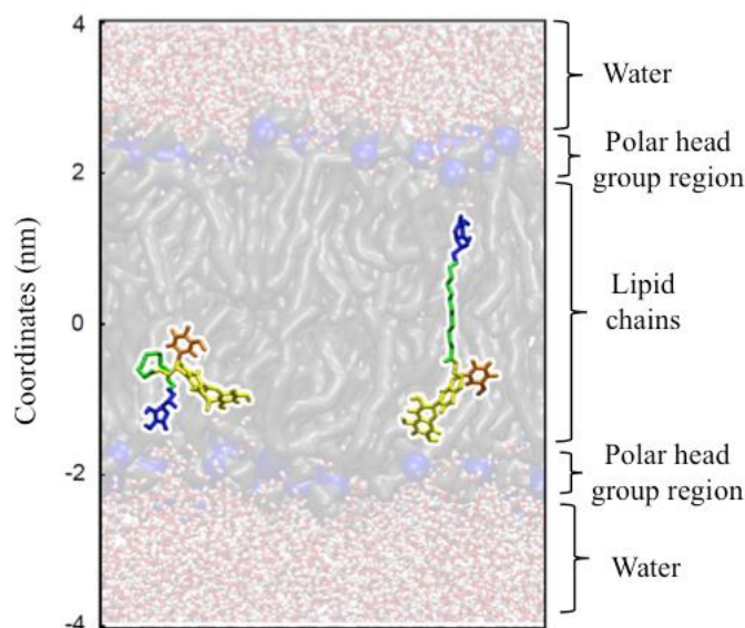
Figure 10. Representative equilibrated location of SB-C 12 -AA in lipid bilayer. Averaged location of a folded (left side) and a linear (right side) conformer over the last 100 ns of 500 ns long MD simulation. AA in blue, linker in green, E-ring of SB in orange and the rest of SB in yellow.
