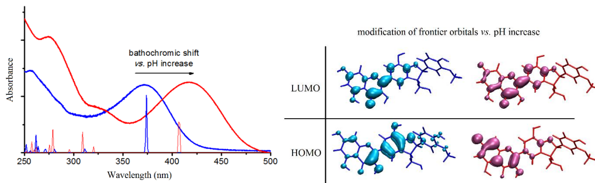
Figure 18. Superimposed theoretical and experimental absorption spectra of DHSCH vs. pH (on the left) and MOs description of the neutral and C7-OH deprotonated form in the first and second column, respectively, on the right. The blue color (spectrum on the left and MOs on the right) corresponds to the neutral form; the red color corresponds to the C7-OH deprotonated form.
