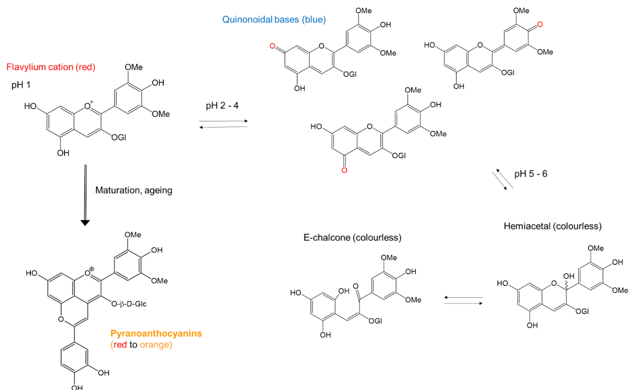
Figure 2. Different forms of anthocyanins vs. pH values
