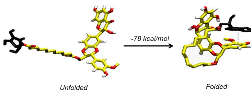
Figure 5. Representative linear and folded conformers of the SB-C 12 -AA conjugate. The AA moiety is in black.
