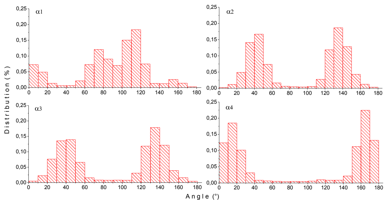
Figure 12. Angles' distribution of malvidin-3- O -glucoside...quercetin system.
