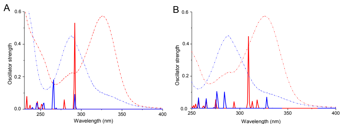
Figure 15. Theoretical spectra of neutral form (in blue) and the C7-OH deprotonated form (in red) of SCH with A) CAM-B3LYP and B) B3P86 functionals. The theoretical and experimental spectra are superimposed, as shown in solid and dashed lines, respectively.
