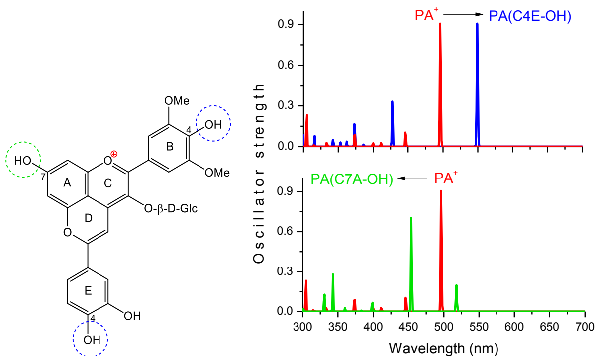
Figure 8. PA1 structure (on the left) and theoretical absorption spectra (on the right). The C7A, C4B and C4E groups are prone to deprotonation. The cation form is in red, C4E-OH and C7A-OH deprotonations shown in blue and green, respectively. The deprotonation at C4B is similar to that at C4E (see Publication IV).
