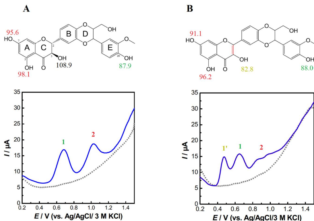
Figure 10. Voltammograms and structures of (A) SB and (B) DHSB. The BDE values of each OH group are expressed in kcal/mol next to the OH groups. The color of the value corresponds to the color of the oxidation peak's number.
