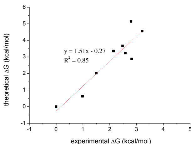
Figure 15. Correlation of theoretical Gibbs energy of association ( \Delta G_{association}^{MM/PBSA} ) vs. experimental energy \Delta G_{association}^{exp} .
