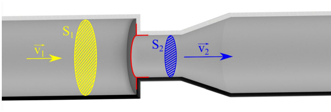
Figure 4.1 Demonstrative pipe (inspired by [33])
