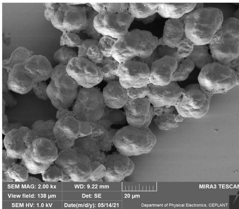
Figure 5.1 PSP of 20 \mu m in size after being exposed to cavitation mode
