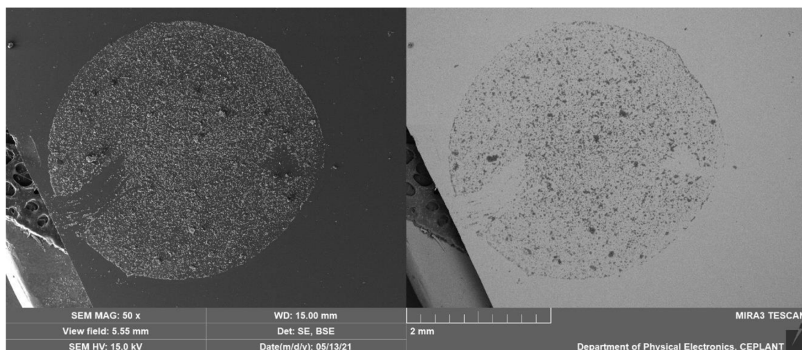
Figure 5.5 A single drop of PSP of 5 μm in size after being exposed to cavitation mode
