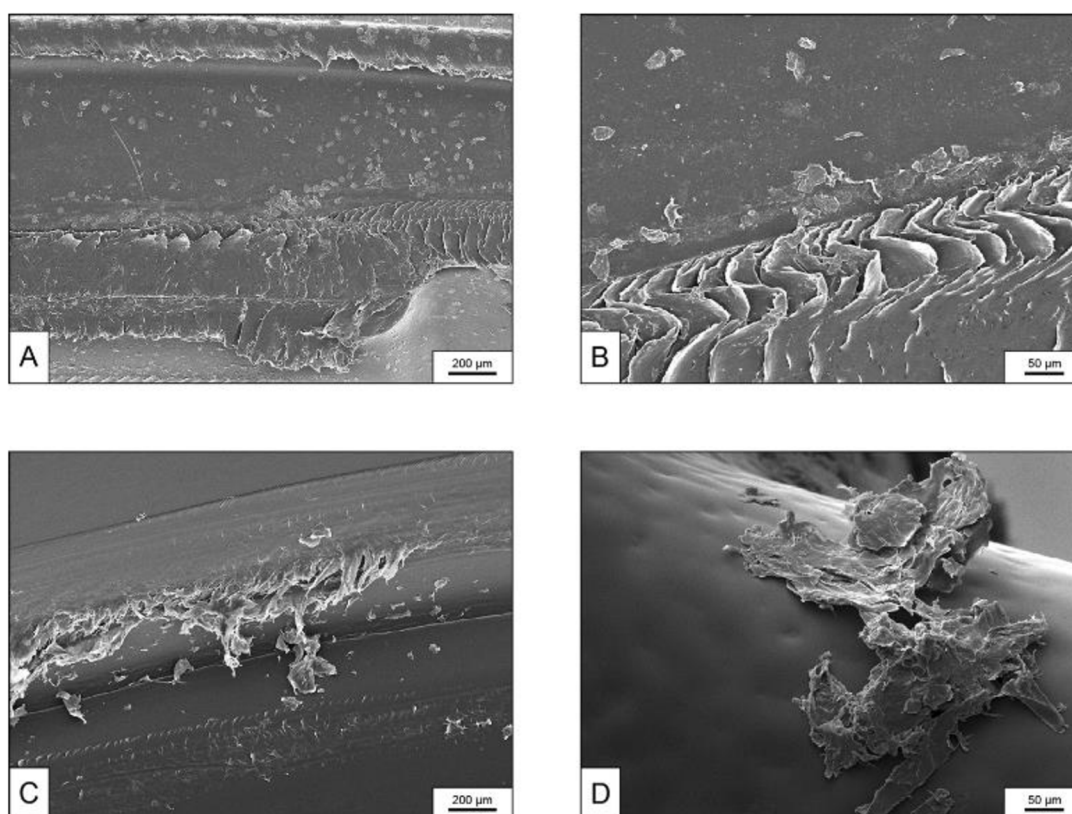
Figure 2.3 SEM images of cap (A-C) and bottleneck (D) of plastic PET bottles after repeated opening/closing procedure (100 x) [23]
