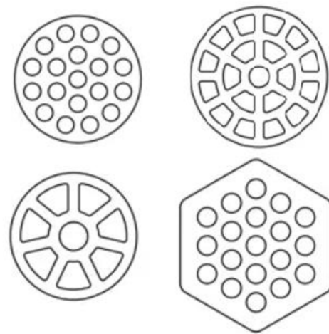
Figure 3.2 Different types of geometry of ceramic filters [28]
