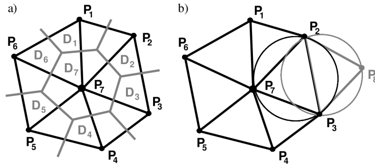
Fig. 3.2 Delaunay triangularization attributes: a) Dirichlet discretization network (grey) and Delaunay discretization network (black), b) the circumscribed circles do not contain any P point.
