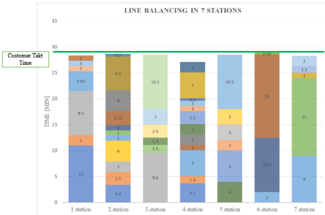
Figure 18:Balancing diagram
