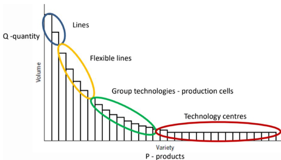
Figure 3: P/Q diagram [3]
