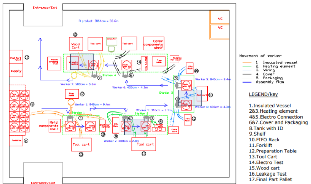
Figure 25: Spaghetti Diagram for Suggested line layout B [Own]
