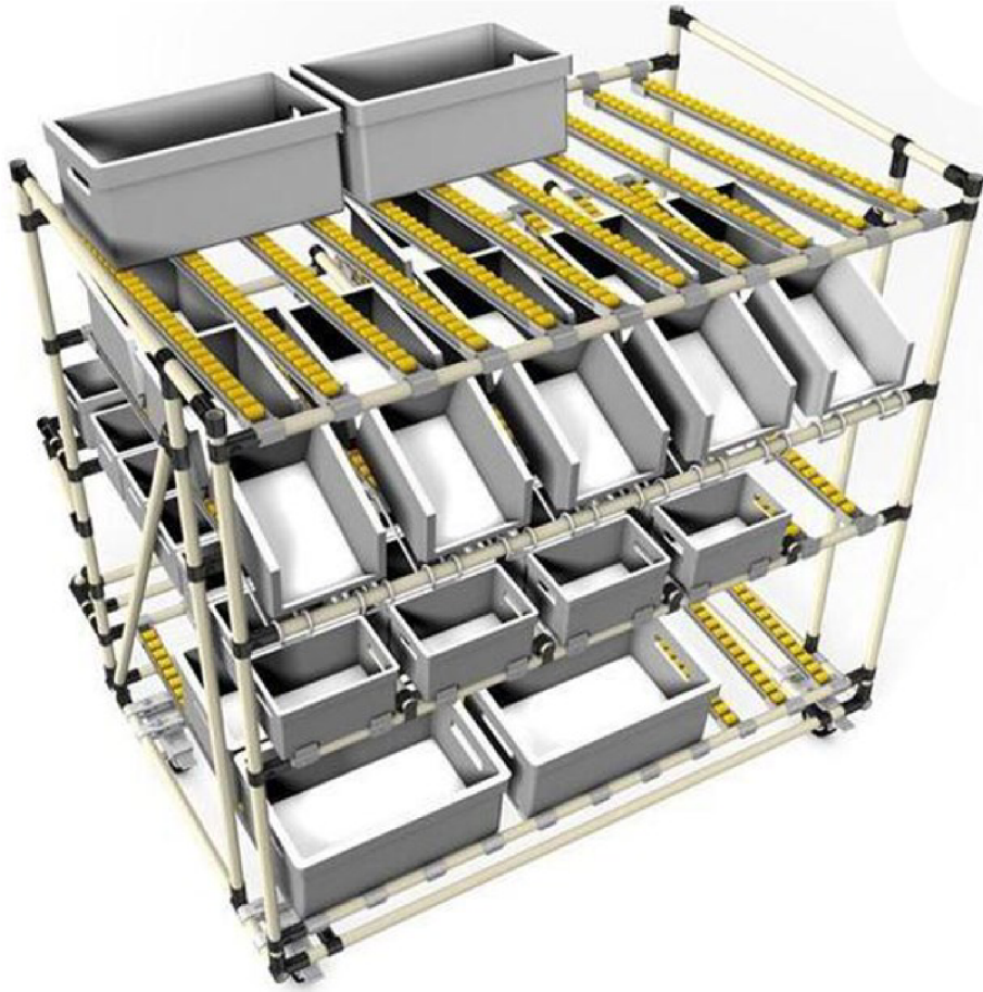
Figure 26:FIFO Rack with Wheels [21]
