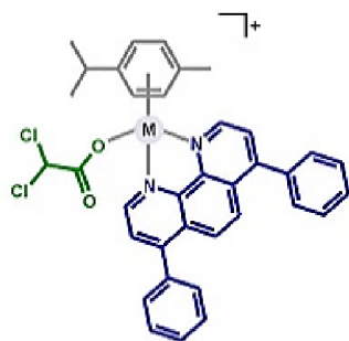
[M(\eta^6\text{-pcym})(\text{bphen})(\text{dca})]\text{PF}_6 M = Ru or Os
