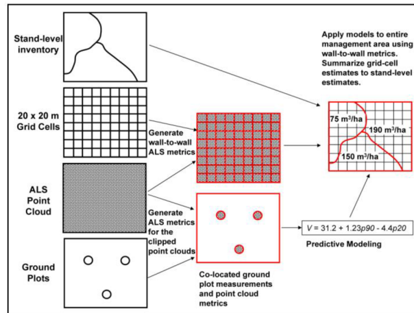
Picture 10 Scheme of the area-based approach; Source - https://www.mdpi.com/forests/forests-04-00518/article_deploy/html/images/forests-04-00518-g001.png
