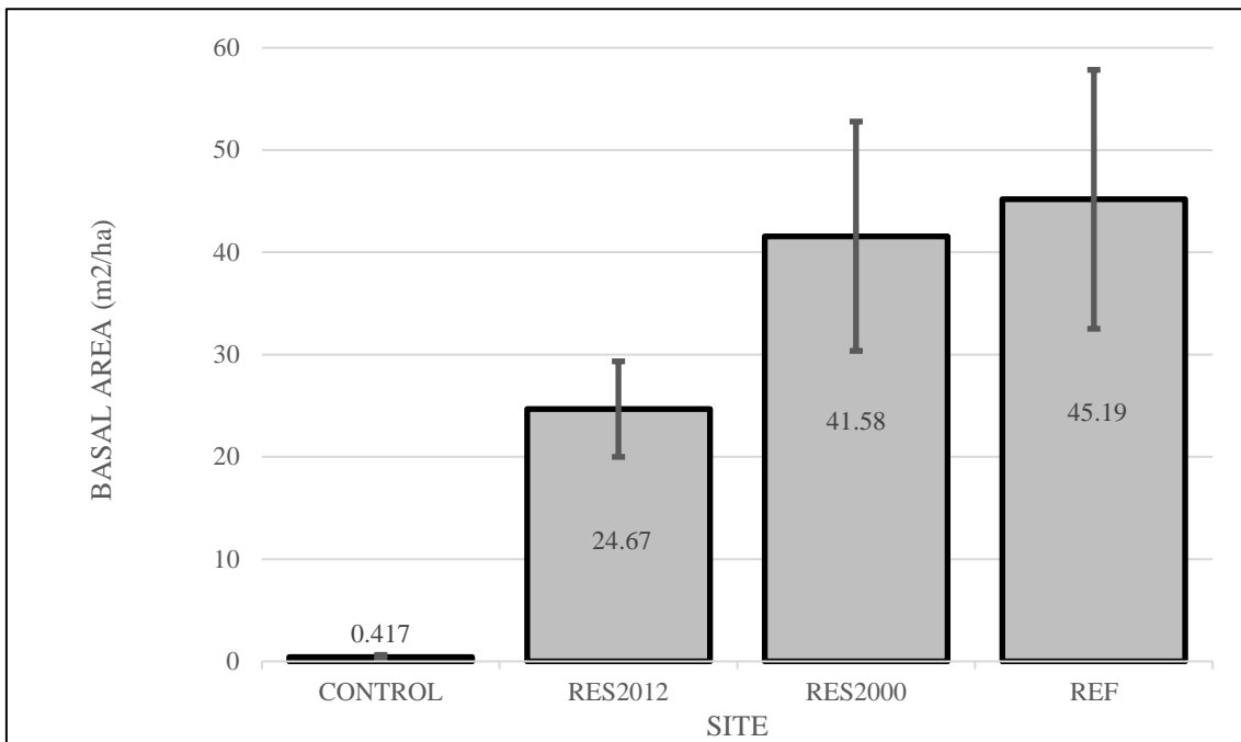
Figure 10. Estimated basal area (m 2 /ha) in all four sites.
