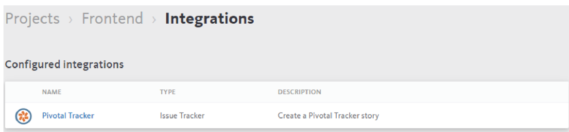
Obr. 5.12: Bugsnag [43]
