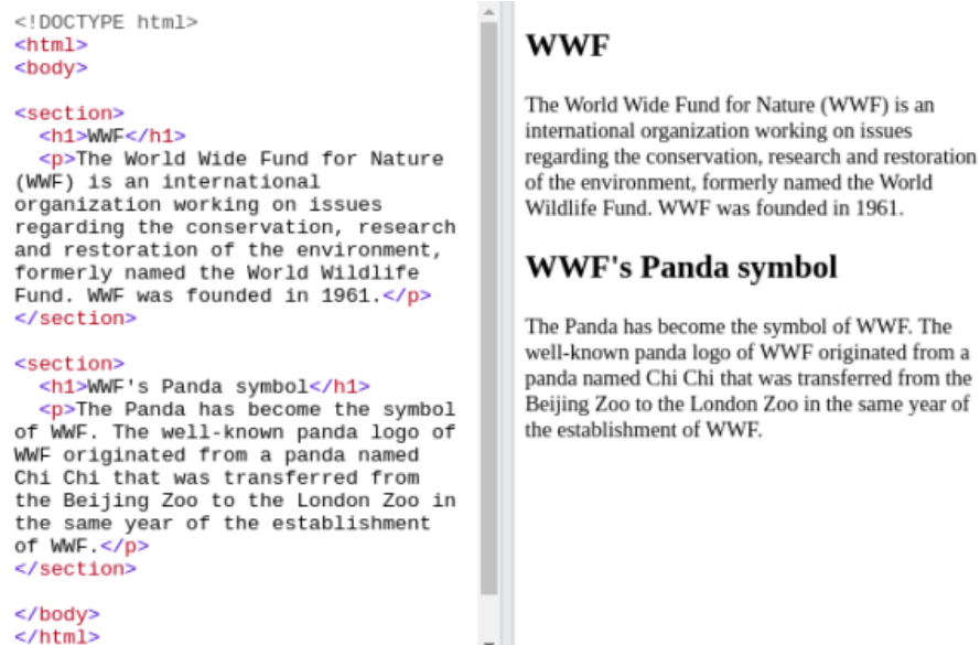
Figure 11. HTML <section> Element. Source:[author]
