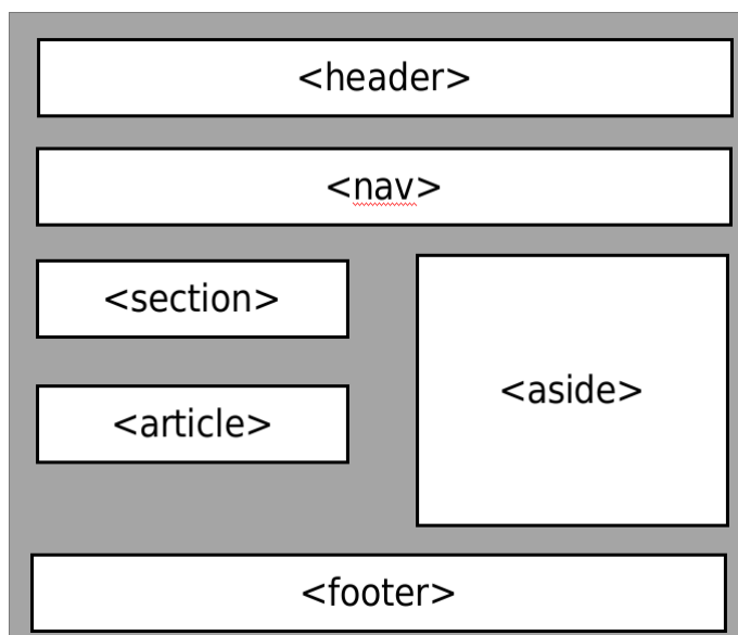
Figure 10. simple HTML Page. Source:[7]
