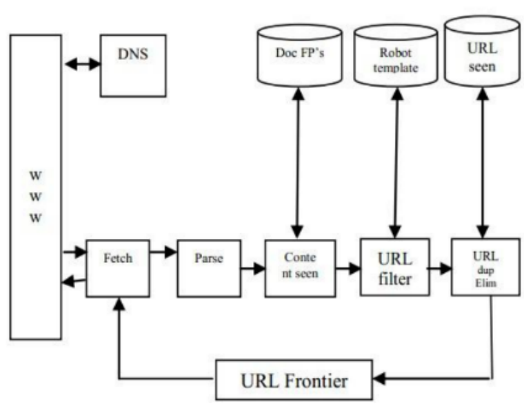
Figure 16. Architecture of a Basic Crawler. Source:[12]
