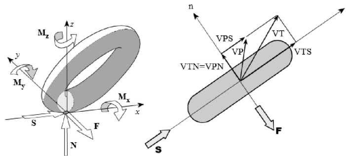
Obr. 6 Model pneumatiky [3]
