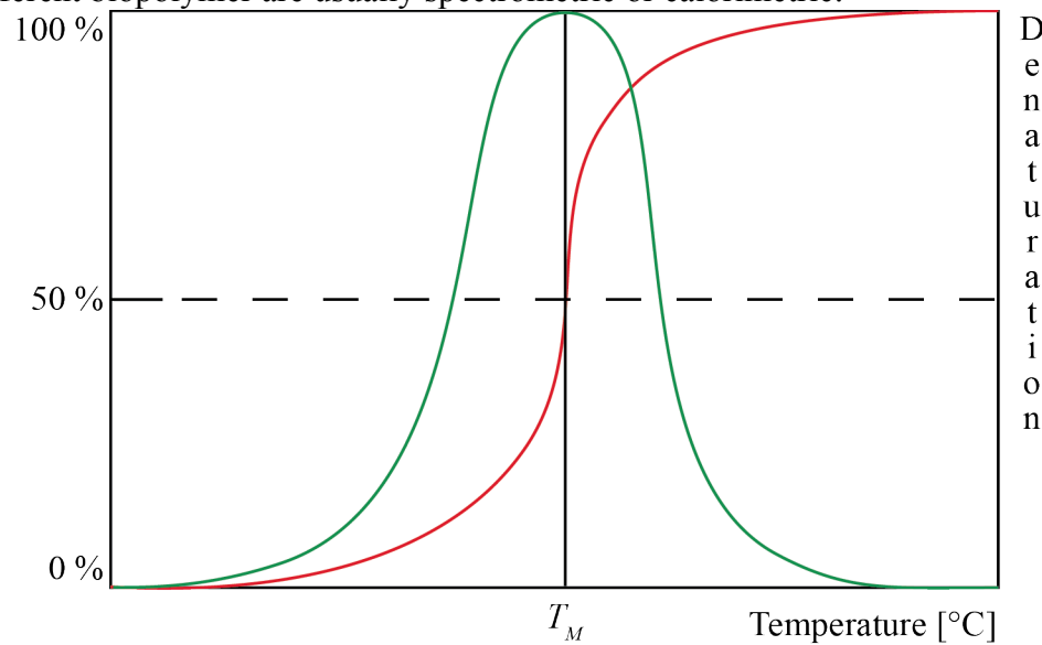
Figure 7: Melting curve
