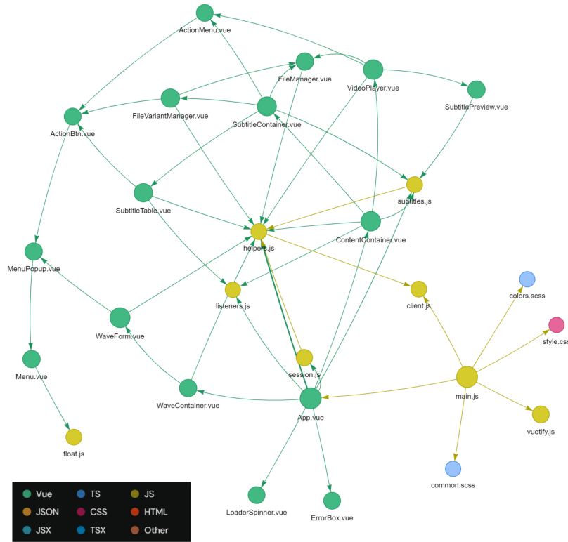
Figure 4.1: Modules's Graph
