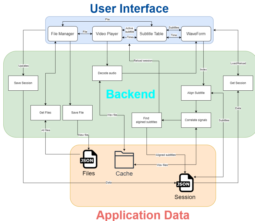
Figure 3.6: Application Schema
