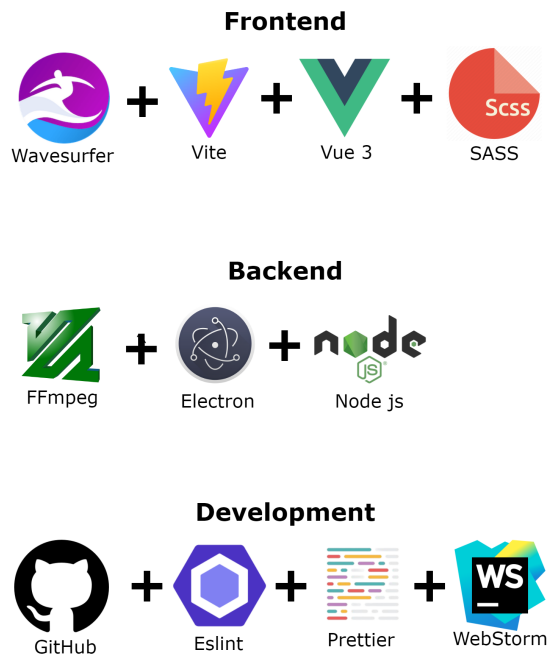
Figure 3.5: Technology stack
