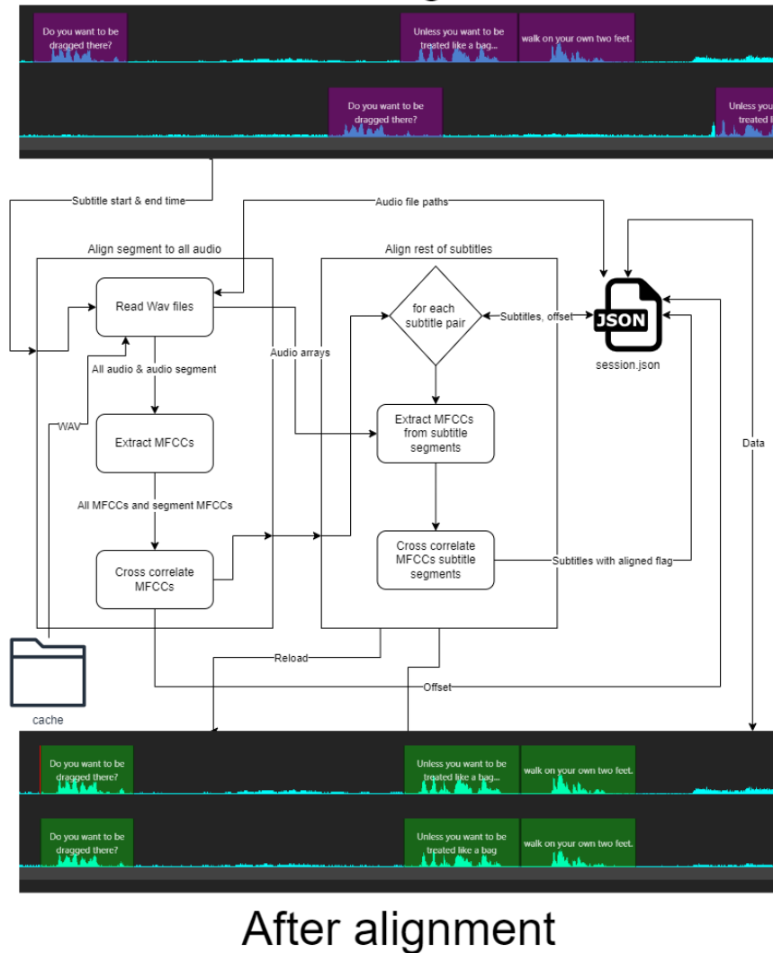
Figure 4.7: Alignment process in the backend
