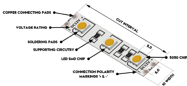
Obr. 2-12 Schéma LED pásku [18]
