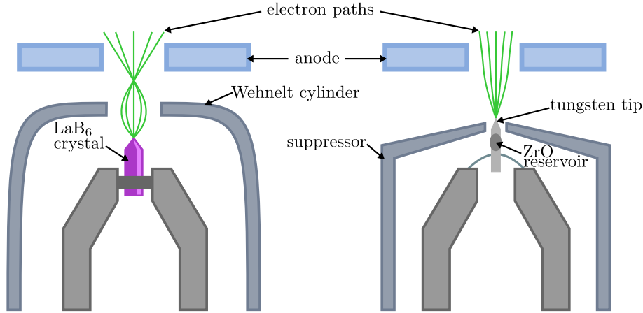
Fig. 1.2: Schematic depiction of a \text{LaB}_6 gun assembly (left) and a Schottky gun assembly (right). The configuration of electrodes in tungsten filament gun assemblies is identical to the \text{LaB}_6 configuration and the electrode configuration of a field emission gun is the same as the Schottky electron gun configuration.
