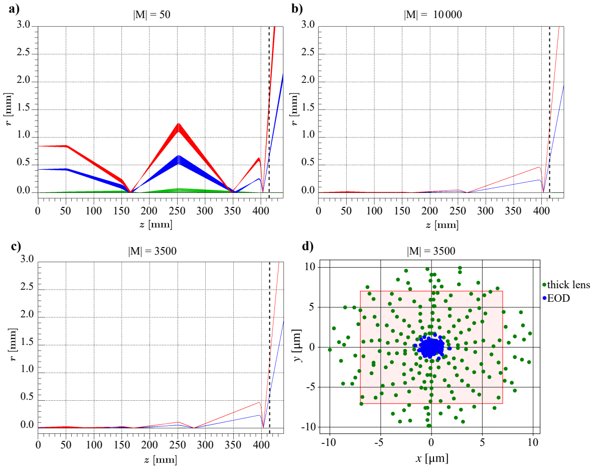
Fig. 4.21: High magnification series particle trajectories for a) |M| = 50 , b) |M| = 10000 and c) |M| = 3500 . The data were obtained using EOD particle tracer. The liner radius is 3.0 \text{ mm} and the dashed black line denotes the position, where the narrow part of the last lens gap ends. d) shows where the particles starting from r = 0.0 \text{ mm} intersect the image plane. Dimensions of the red rectangle correspond to the size of a single 14 \mu\text{m} \times 14 \mu\text{m} pixel.
