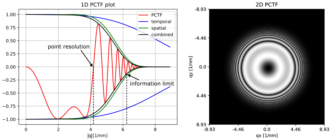
Fig. 1.19: The magnitude of the 2D PCTF at Scherzer defocus on the right and the respective 1D PCTF on the left. Following parameters were used to obtain these graphs: spherical aberration coefficient C_{3,0} = 1.2 mm, chromatic aberration coefficient C_C = 1.2 mm, acceleration voltage U = 200 kV, root-mean-square energy spread \Delta E_{\text{rms}} = 0.7 eV, HT ripple \Delta U = 0.1 V, lens current stability \frac{\Delta I}{I} = 0.5 ppm and illumination aperture \alpha = 0.3 mrad.
