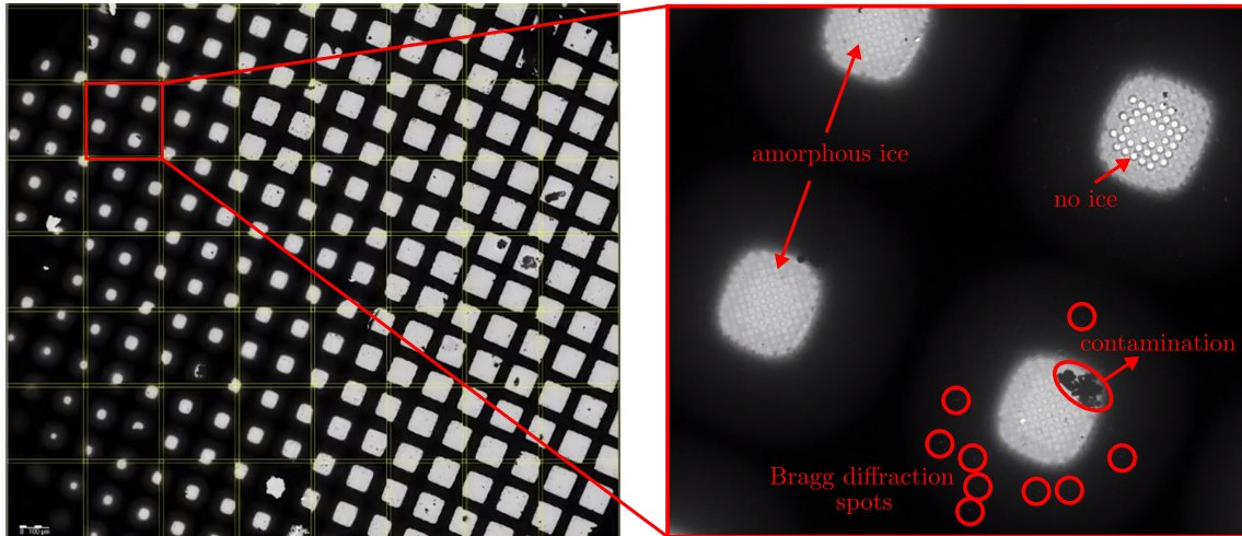
Fig. 3.4: A map of vitrified is shown on the left and its detail on the right.
