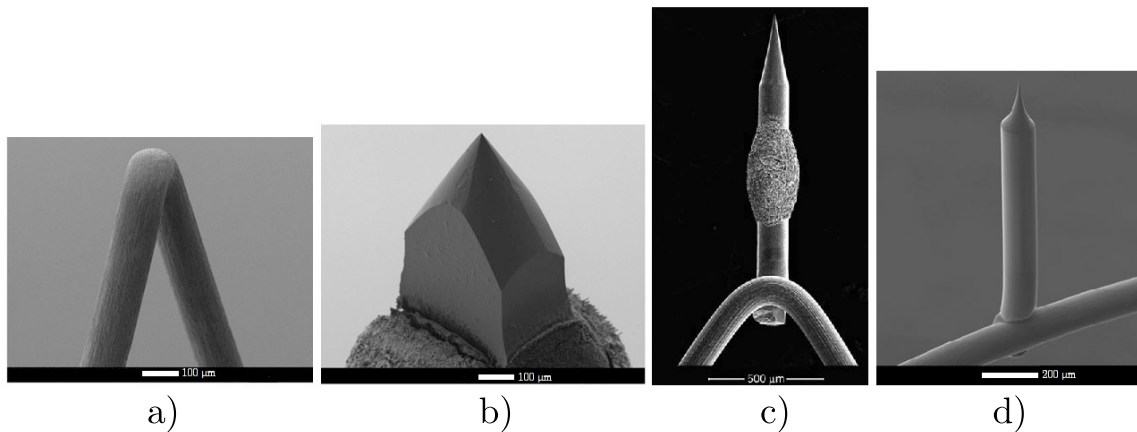
Fig. 1.3: a) Tungsten filament emitter, from [15]. b) \text{LaB}_6 emitter [15]. c) Schottky emitter, a tungsten monocrystal with a zirconium oxide reservoir attached to a tungsten filament, from [14]. d) Cold field emitter, a tungsten monocrystal attached to a tungsten filament, from [15].
