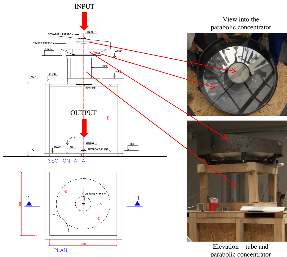
Fig. 4.1: Chamber (plan, elevation) and photographs of the light guide concentrator
