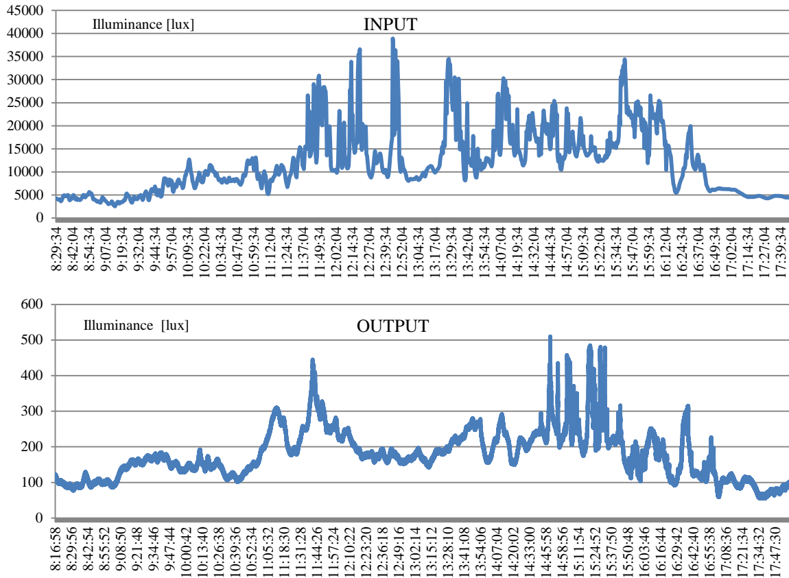
Fig. 5.2: Daily profiles of illuminance on the input and output of the light guide for cloudy sky daylight illuminance, 02/05/2015
