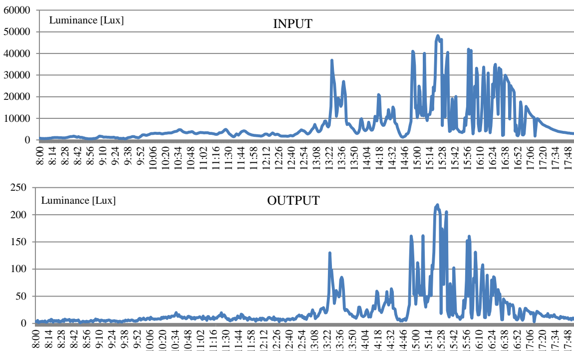
Fig. 5.3: Daily profiles of illuminance on the input and output of the light guide for dynamic changes of daylight illumination, 23/06/2015
