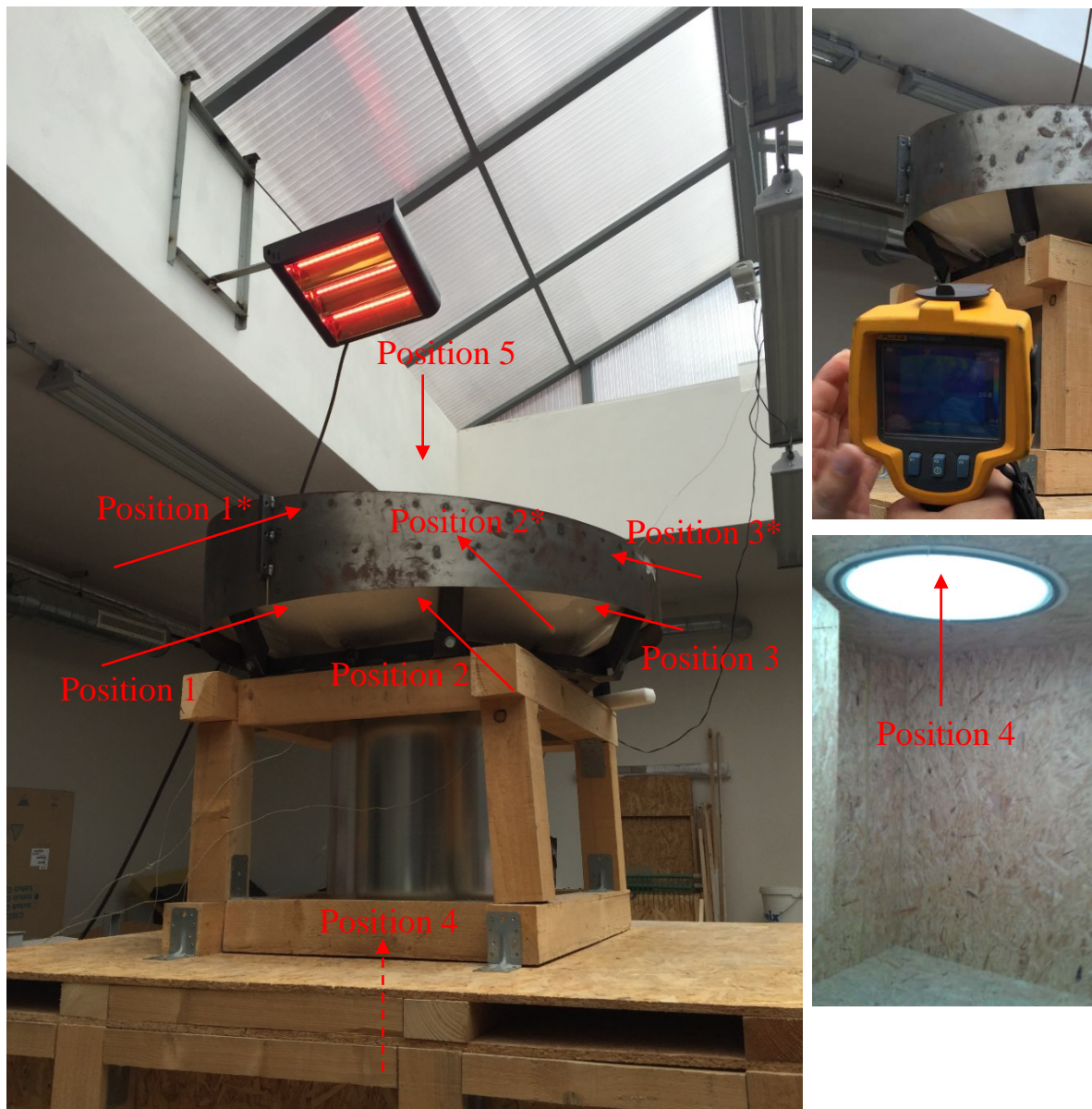
Fig. 4.2: Photograph of the light guide under the IR lamp radiation and view to the light guide diffuser (inside the chamber)
