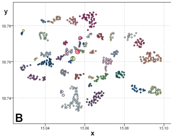
Min Samples = 30
