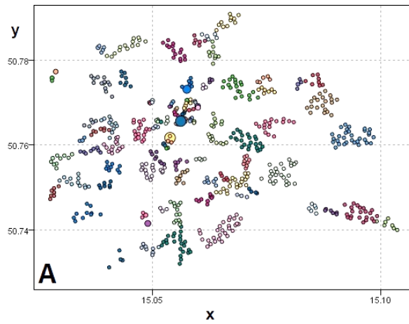
Min Samples = 10
