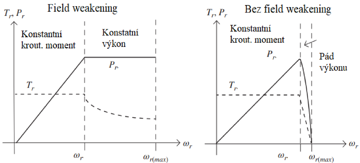
Obr. 10 - Field weakening [7]
