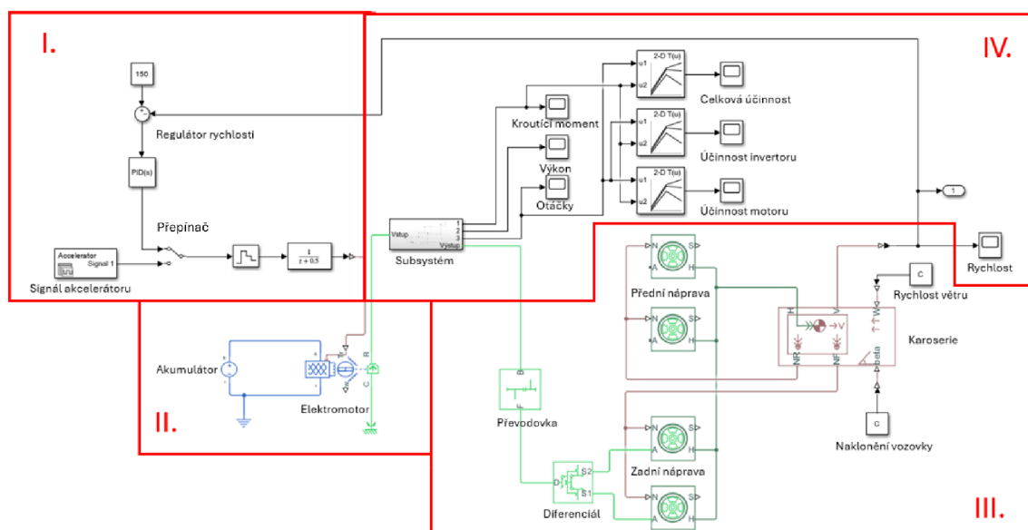
Obr. 18 - Simulink model
