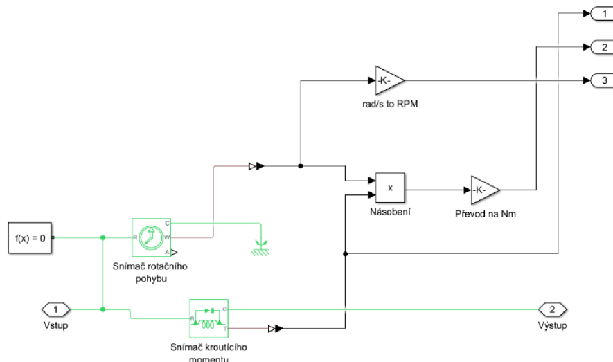
Obr. 20 – Podsystem modelu
