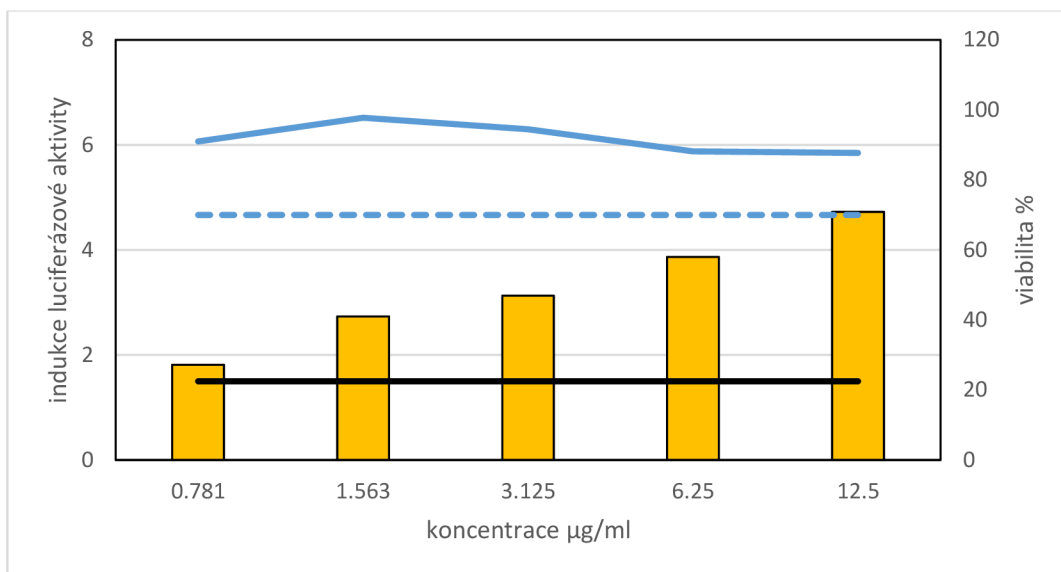
Graf. 13: Butyl-4-hydroxybenzoate
