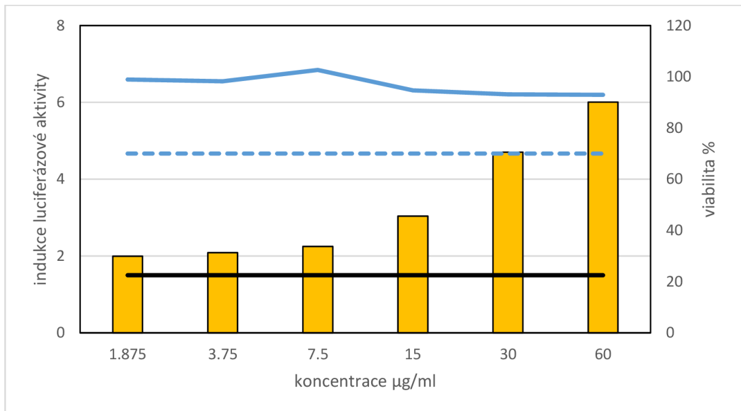
Graf. 12: Ethyl-4-hydroxybenzoate
