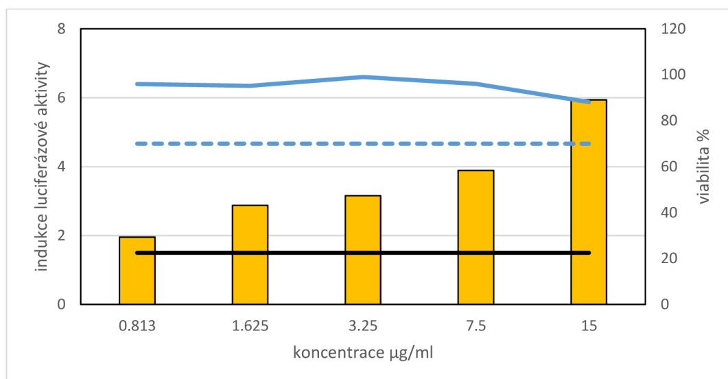
Graf. 14: Isobutyl-4-hydroxybenzoate
