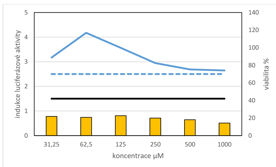
Graf. 7: Tartrazine
