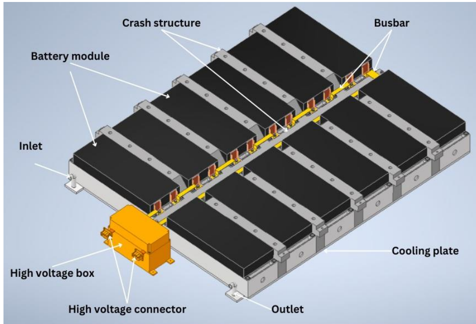
Figure 42 : Components inside the battery box
