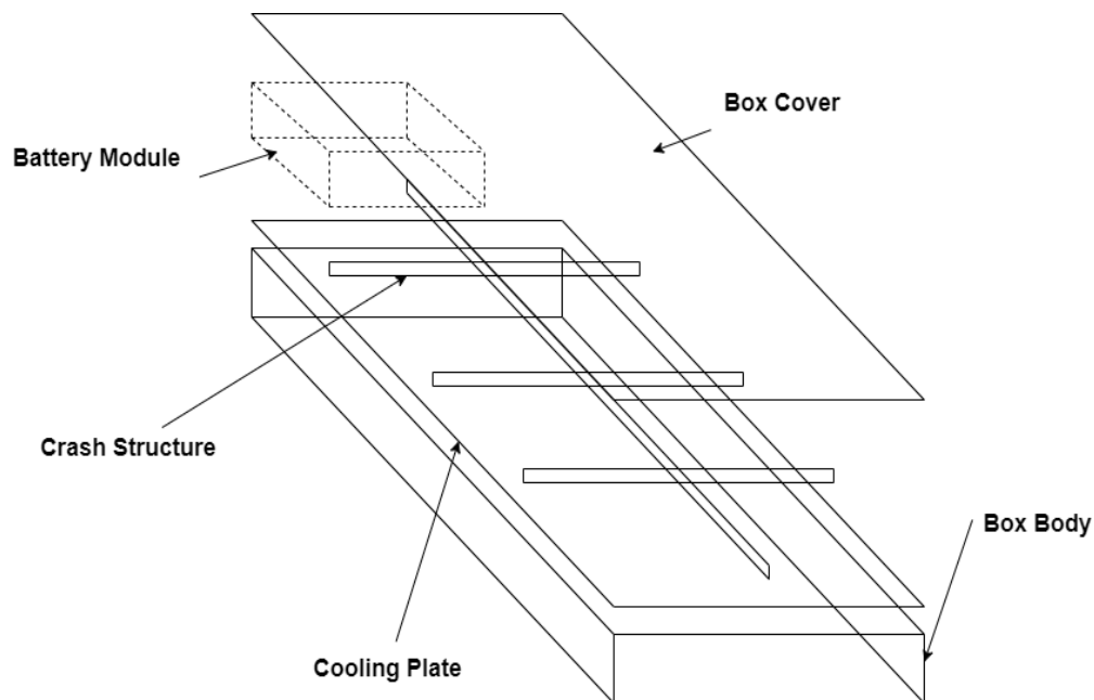
Figure 36 : Concept 2
