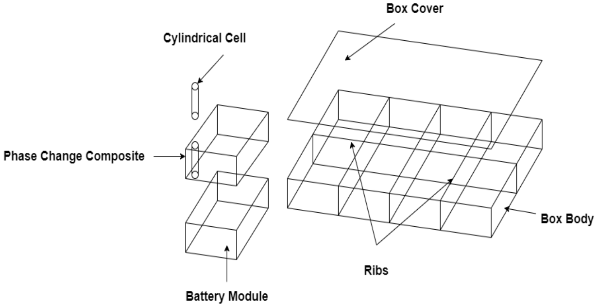
Figure 38 : Concept 4
