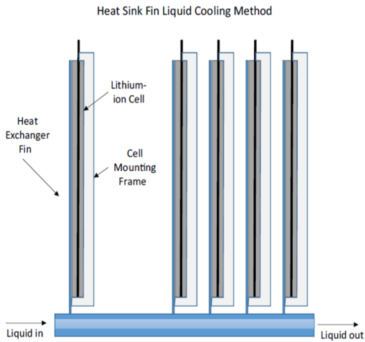
Figure 7 : Heat sink fins [8]
