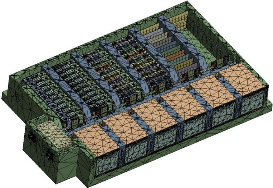
Figure 52 : Mesh generation
