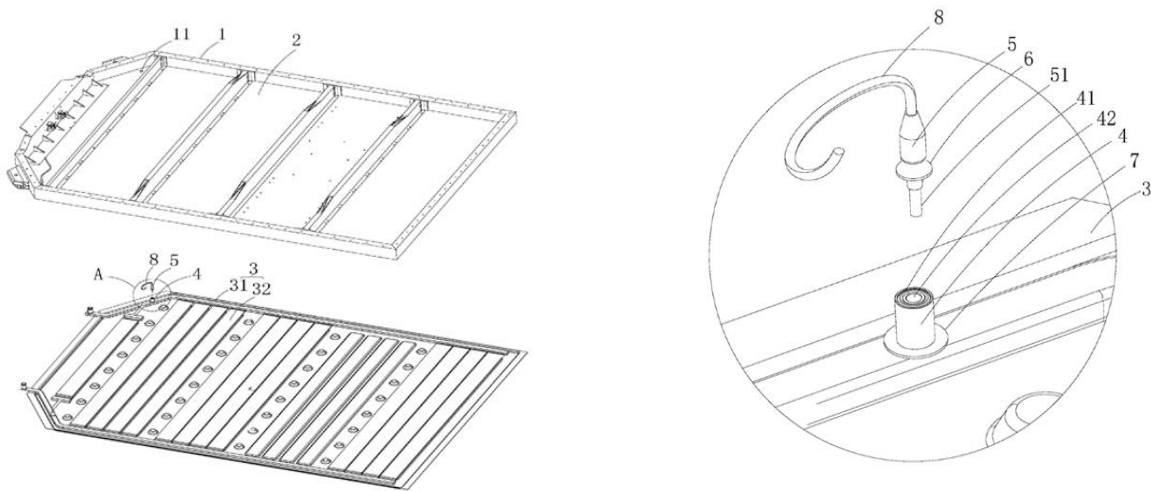
Figure 15 : Document CN213782095U [19]
