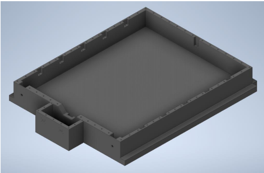
Figure 41 : Battery box body from composite material
