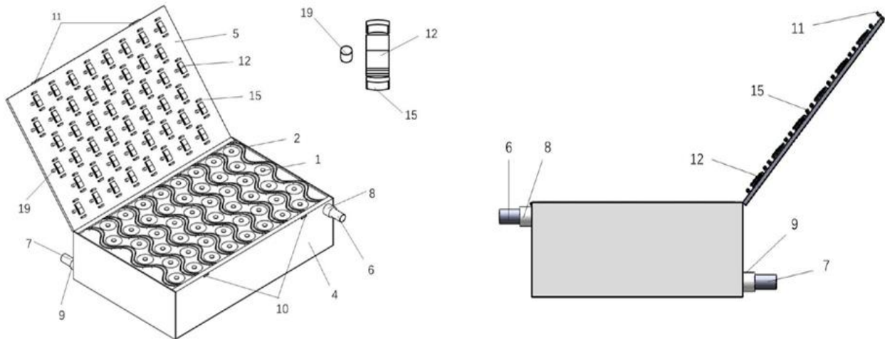
Figure 21 : Document CN113314783A [19]
