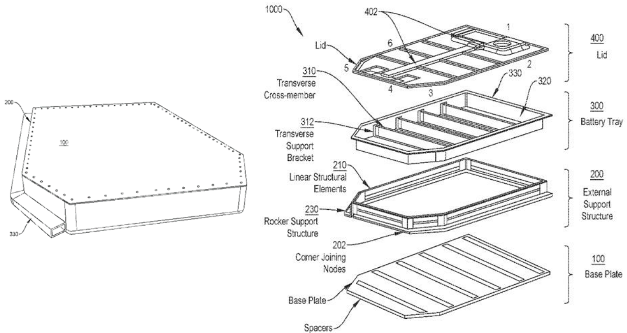
Figure 16 : Document US2021323418A1 [19]
