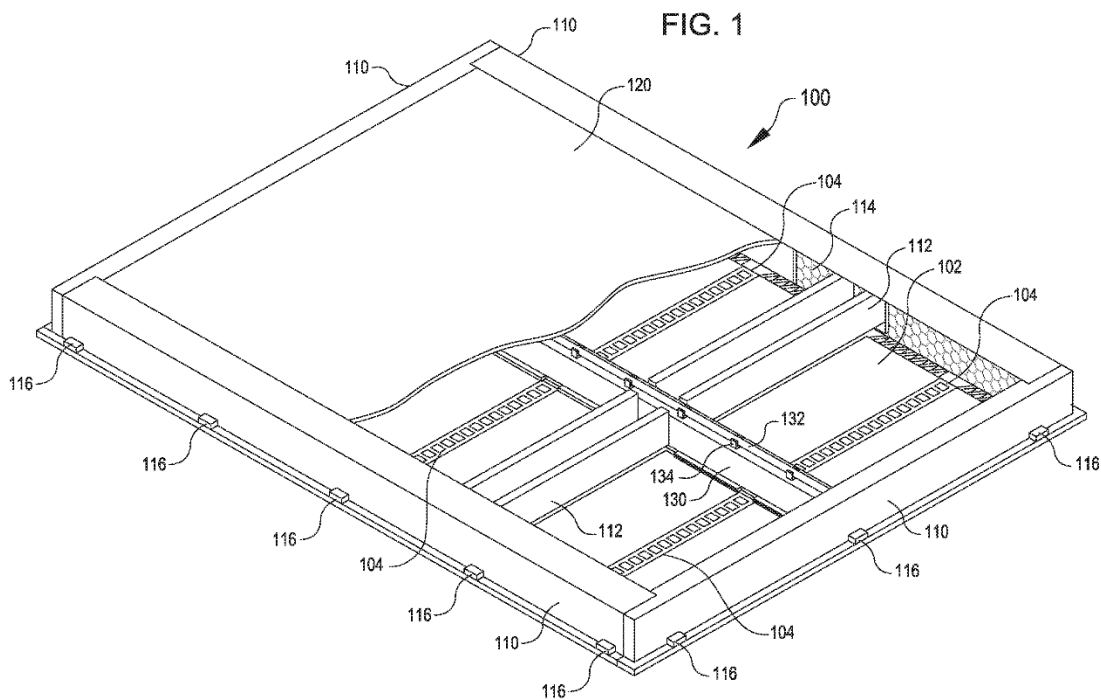
Figure 17 : Document US2021305544A1 [19]
