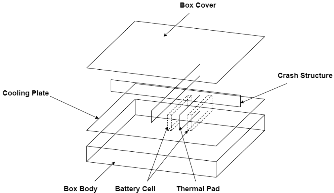
Figure 39 : Concept 5
