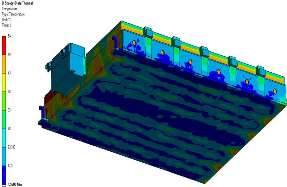
Figure 53 : The temperature field outside the battery modules with the cooling system
