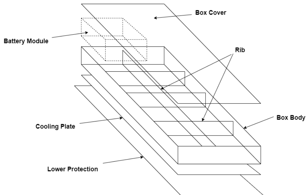
Figure 35 : Concept 1
