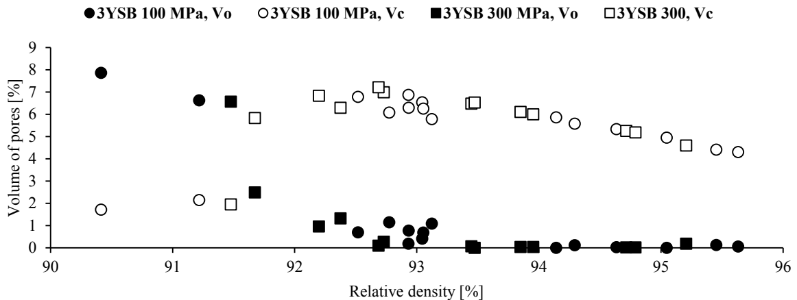
Figure 35: Evolution of porosity for 3YSB 100 MPa and 300 MPa CIP.
