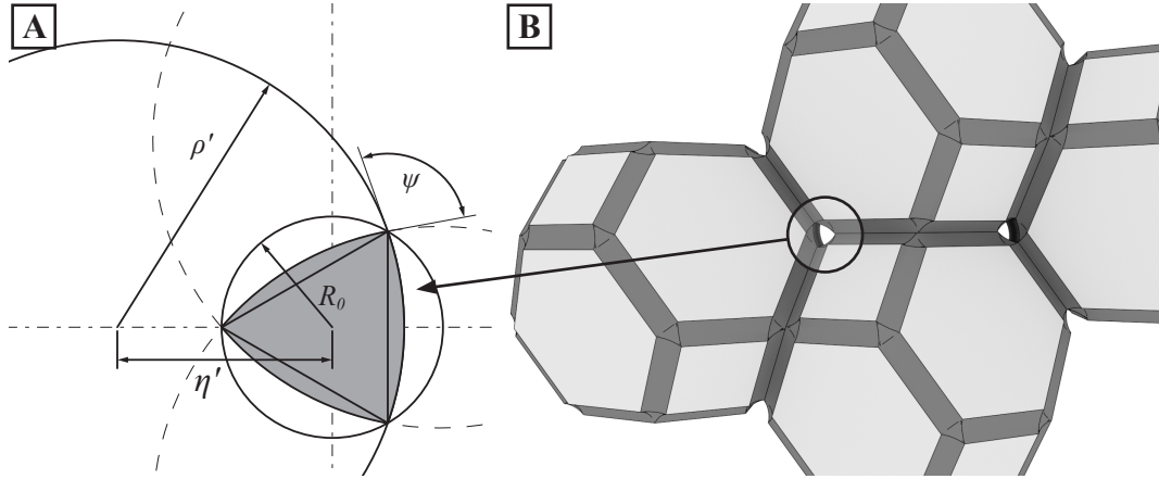
Figure 19: A) Geometry of idealised three-sided pores.
