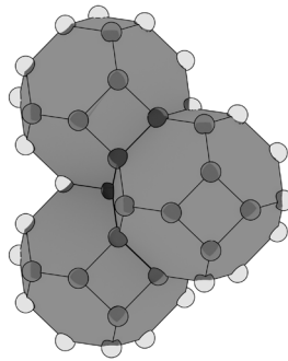
Figure 21: Idealised model of grains for the third stage of sintering with spherical pores on grain corners.
