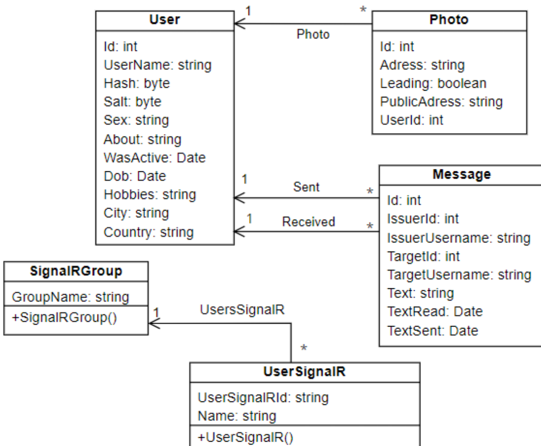
Figure 10.UML Class diagram
