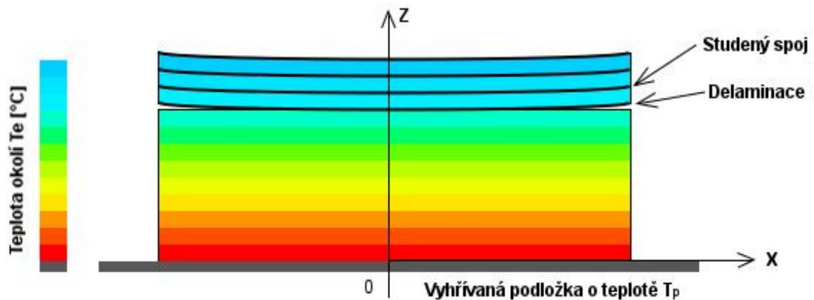
Obr. 2-22 Delaminace.
