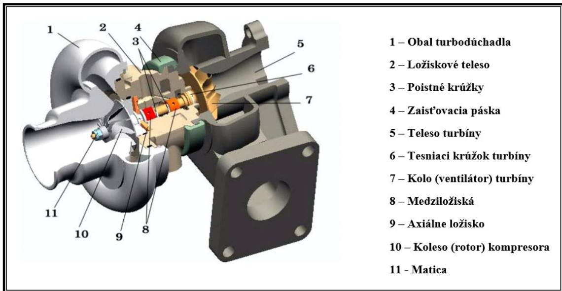
Obr. 3.3 Prierez turbom
