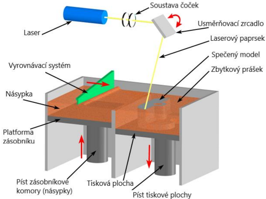
Obr. 13 Technologie DMLS [41].
