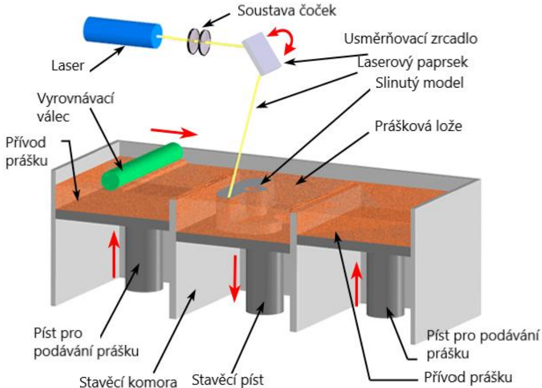
Obr. 12 Technologie SLS [38].
