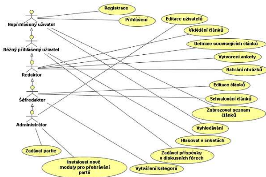
Obr. 1: UseCase diagram
